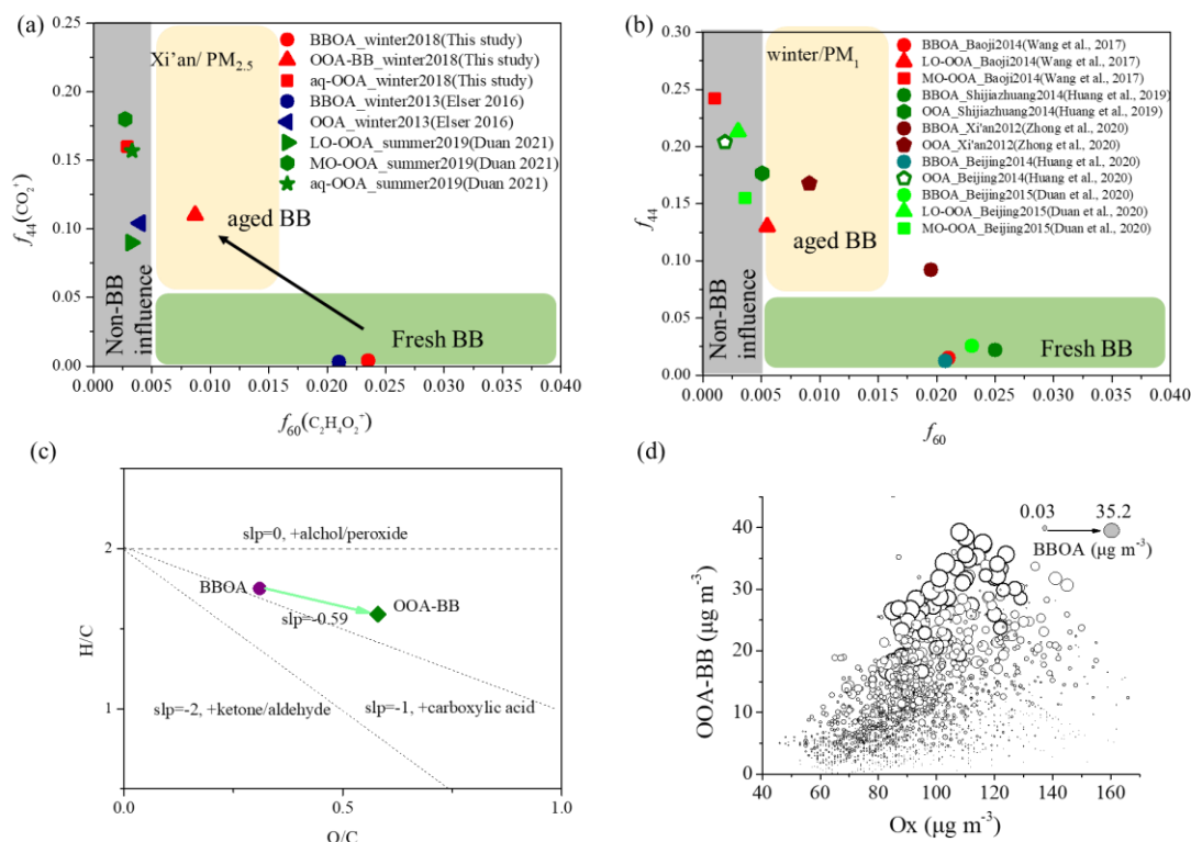
Fig. 3 f_{44} vs. f_{60} for BBOAs and SOAs resolved in OA of PM_{2.5} in Xi'an (a); f_{44} vs. f_{60} for BBOAs and SOAs resolved in OA of PM_1 in our previous campaigns conducted in Xi'an, Baoji, Shijiazhuang and Beijing (b); the van Krevelen (VK) diagram of the BBOA and OOA-BB factors resolved in the winter of 2018 in Xi'an (c); and the effects of Ox and BBOA concentrations on the OOA-BB formation (d).
