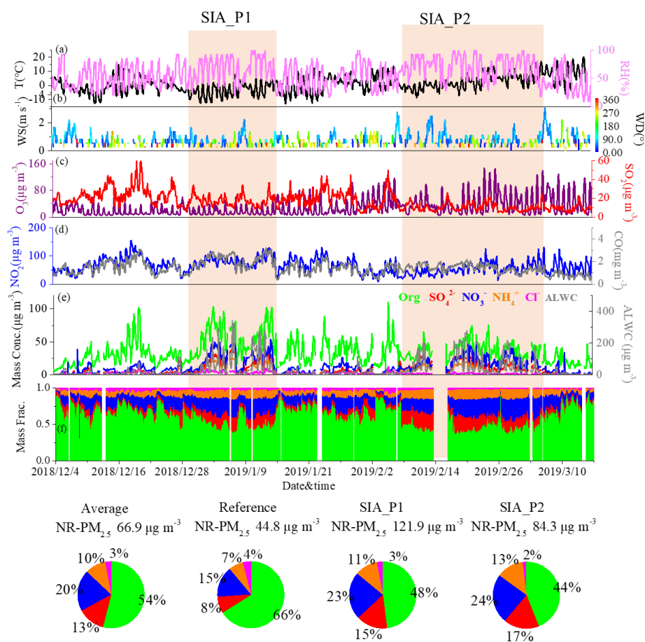
Fig. 1 Time series of meteorological parameters (relative humidity (RH), temperature (T), wind speed (WS), and wind direction (WD) (a, b); gases (SO 2 , O 3 , NO 2 and CO) (c, d); and NR-PM 2.5 composition as well as the aerosol liquid water content (ALWC) (e, f) in the winter of 2018 in Xi'an. The average composition of NR-PM 2.5 for the entire winter campaign, as well as reference days and SIA-enhanced periods (SIA_P1 and SIA_P2) are also shown.
