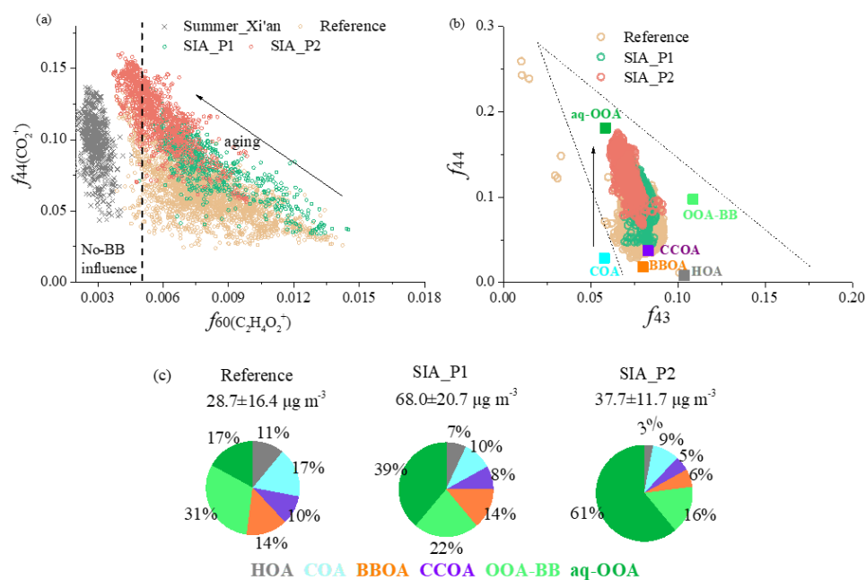
Fig. 4 f_{44} vs f_{60} during three periods including reference days, SIA_P1, and SIA_P2, f_{44} vs f_{60} in summer 2019 was also shown for comparison (a), f_{44} vs f_{43} during these three periods, the corresponding values of the six OA factors identified in this study are also shown, and the triangle range is from Ng et al. (2010) (b), and the average OA concentration and composition during these three periods (c).
