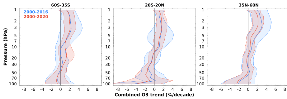
Figure 3. Combined post-2000 ozone profile trend estimates and uncertainties (2-sigma) from the seven merged satellite records (below the 50 hPa level: five records, see text). Red (blue) solid line and light red (blue) shaded areas indicate LOTUS22 (LOTUS19) trend values and uncertainties.
