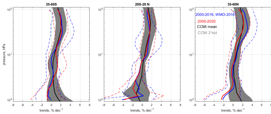
Figure 5. Black line: multi-model mean ozone profile trend estimates from the CCMi REF-C2 simulations over three broad latitude bands (left 60°S – 35°S, center 20°S-20°N, right 35°N- 60°N). Grey envelope: 2 \sigma uncertainty of the multi-model mean trend estimates. Red (blue) lines and light red (light blue) dashed lines represent LOTUS22 (LOTUS19) average and 2-sigma uncertainty respectively.
