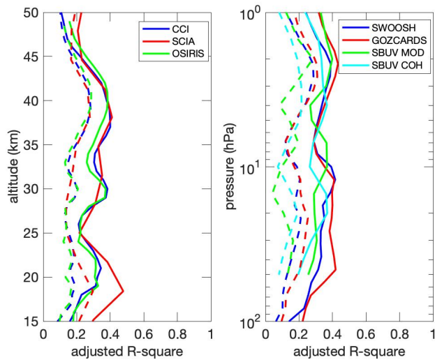
Figure 7. Adjusted R^2 values of the LOTUS regression model using seasonal (solid lines) and non-seasonal (dashed lines) variation of fitted coefficients in the LOTUS regression model (see text).
