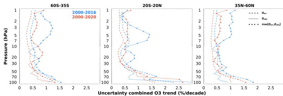
990 Figure 6. Decomposition of error terms for the combined trend estimates: propagation of errors from fit residuals ( \sigma_{\text{err}} , dashed lines) and standard error of the trend sample ( \sigma_{\text{obs}} , dotted lines) for LOTUS22 in red and LOTUS19 in blue for the three broad latitude bands. Combined trend uncertainty is shown by circle symbols that indicate the maximum of \sigma_{\text{err}} and \sigma_{\text{obs}} in each case.
