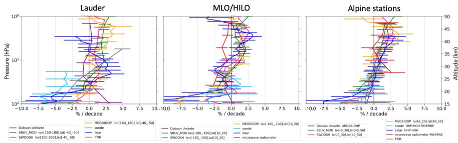
Figure 4. Ozone profile trends for the post-2000 periods from selected ground-based NDACC stations. Left panel: SH Lauder station, middle panel: Tropical Mauna Loa and Hilo (ozonesondes) stations, right panel: NH Alpine stations (see text)
