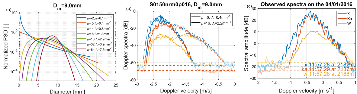
Figure 12. (a) Gamma PSDs with D_m of 9 mm and various shape parameters \mu (see the legend for numeric values). (b) Corresponding Doppler spectra at X, Ka and W-band (see color key in panel (c)) forward-modeled using the SSRGA-plates- \mathcal{M}0.016 model, for an exponential PSD ( \mu = 0 , thin line) and a narrow PSD ( \mu = 16 , thick line). (c) Examples of observed Doppler spectra where similar D_m and \mu are suggested by the retrieval using the SSRGA-plates- \mathcal{M}0.016 model (see Fig. 11). In (b) and (c), the horizontal dashed lines represent the noise level estimated from each Doppler spectra and the portions of lines with weak color saturation highlight the parts of the Doppler spectra which are identified as noise.
