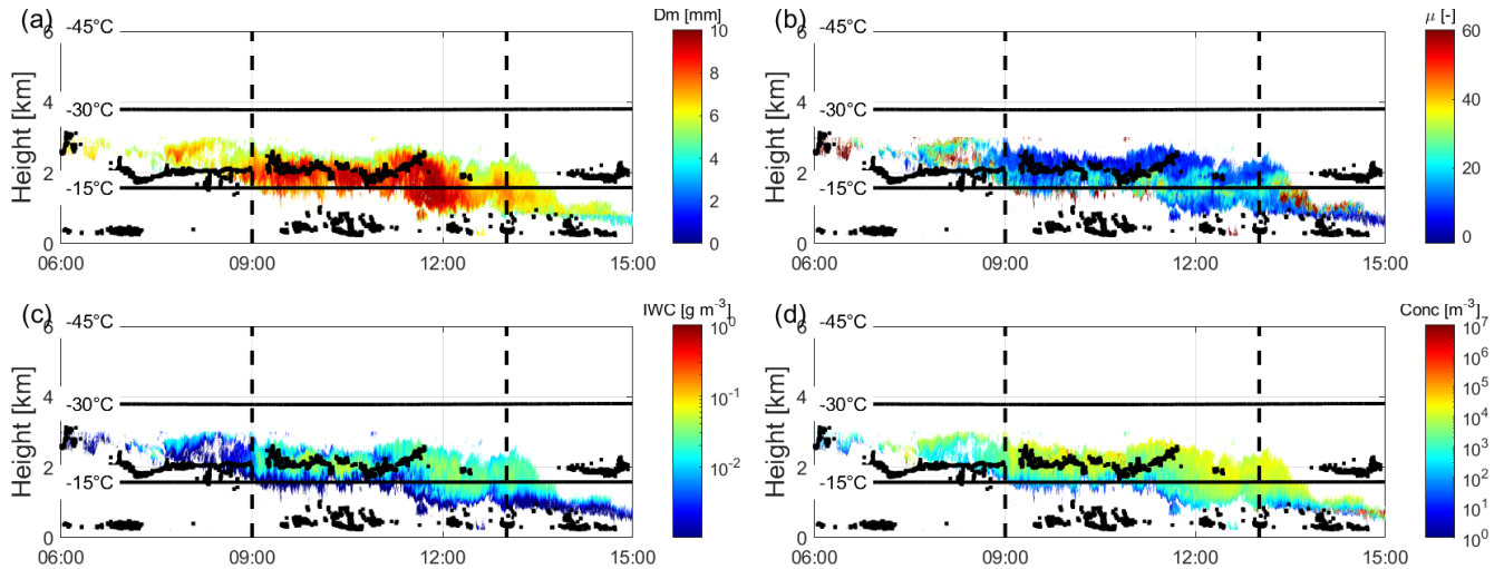
Figure 10. Time height cross section of the retrieved (a) D_m , (b) \mu , (c) IWC and (d) N_i when using the SSRGA-plates- \mathcal{M}0.016 model, for all pixels where \text{DWR}_{K_a, W} is larger than 4 dB. The black dots show the location of supercooled liquid water as detected by the ARM high spectral resolution lidar.
