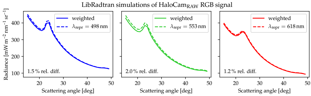
Figure B3. Radiative transfer simulations performed with libRadtran for the HaloCam RAW red, green and blue channel in the principal plane above the sun with SZA = 45^\circ . A cirrus cloud with COT = 1 (at a wavelength 550 nm), r_{\text{eff}} = 20 \mu\text{m} and a mixture of 25% smooth and 75% severely roughened solid columns was assumed. The continental average aerosol mixture from OPAC was chosen with AOT = 0.1 at 550 nm.
