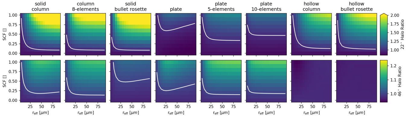
Figure 2. Sensitivity of the halo features, represented here by the 22^\circ (upper panel) and 46^\circ halo ratio (lower panel), to ice crystal shape, effective radius ( x -axis), and smooth crystal fraction (SCF) ( y -axis) based on the look-up tables (LUTs) used for the retrieval. These features are a selection of the full LUT for a wavelength of 618 nm, SZA = 40^\circ , AOT = 0.25, COT = 1.0, and image segment no. 1 (cf. Fig. 4). The white contour lines mark the threshold assumed here for a visible 22^\circ or 46^\circ halo at halo ratio HR = 1.
