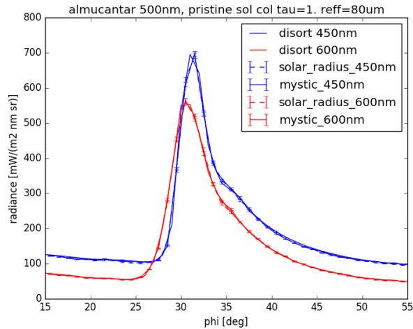
Figure A1. Comparison between MYSTIC (lines with error bars) and DISORT (solid lines) for the region of the 22^\circ halo for red (600 nm) and blue light (450 nm). For the MYSTIC simulations, the effect of taking the solar radius into account (dashed lines with error bars) vs. assuming a point source (solid lines with error bars) is shown as well. 10^5 photons are used for the MYSTIC simulations and 16 streams for DISORT. For all simulations a solar zenith angle of 50^\circ is assumed and the halo slice is computed in the almucantar plane, i.e. with varying azimuth and constant solar zenith angle. The ice cloud was defined with an optical thickness of 1 and consists of smooth solid columns with an effective radius of 80 \mu\text{m} .
