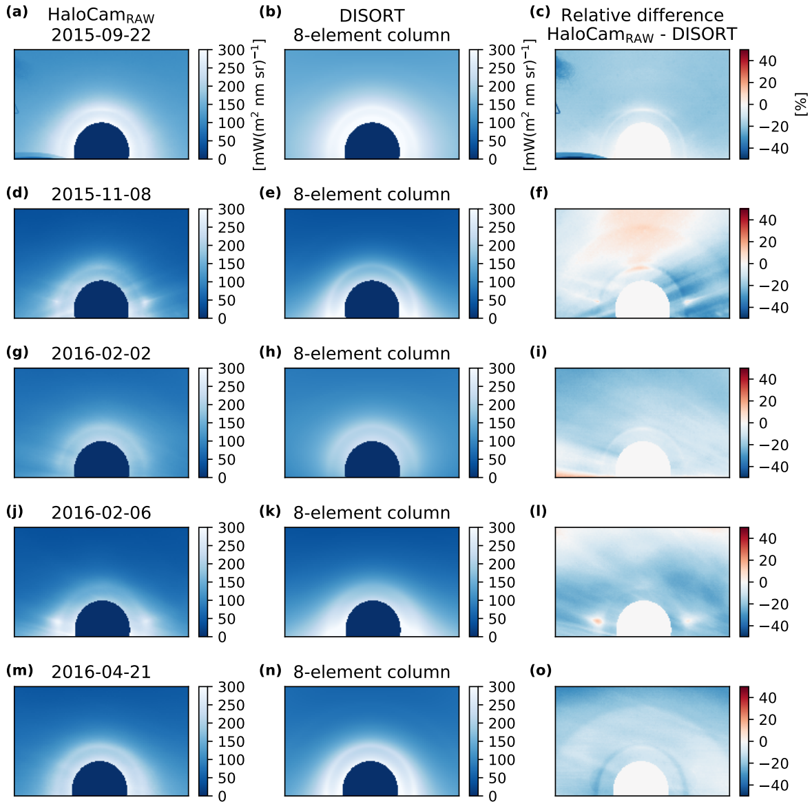
Figure 9. Same as Fig. 8, for selected days and for 8-element columns, the overall best matching ice crystal habit for both the 22° and 46° halo region.
