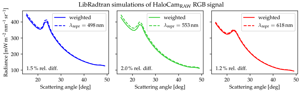
Figure B3. Radiative transfer simulations performed with libRadtran for the HaloCam RAW red, green and blue channel in the principal plane above the sun with SZA = 45°. A cirrus cloud with COT = 1 (at a wavelength 550 nm), r_{\text{eff}} = 20 \mu\text{m} and a mixture of 25% smooth and 75% severely roughened solid columns was assumed. The continental average aerosol mixture from OPAC was chosen with AOT = 0.1 at 550 nm.
