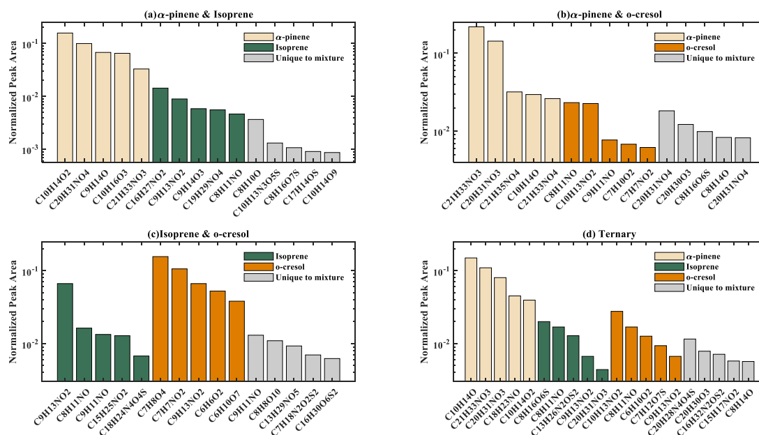
Figure 7: The dominant compounds in terms of their normalized peak area in the mixed VOC systems shown in the bars: (a) binary \alpha -pinene / Isoprene system; (b) binary \alpha -pinene / o -cresol; (c) binary Isoprene / o -cresol; (d) ternary system respectively. The normalized peak area of these selected compounds in a mixed precursor's system are also presented if they existed in corresponding single precursor's system (yellow: single \alpha -pinene, green: isoprene, orange: o -cresol). The compounds are considered identical in the mixed system and single VOC systems if they have the same empirical formula and a retention time difference of <0.1min in positive ionization mode.
