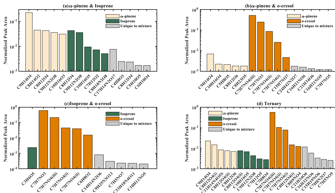
875 Figure 6: The dominant compounds in terms of their normalized peak area in the mixed VOC systems shown in the bars: (a) 880 binary \alpha -pinene / Isoprene system; (b) binary \alpha -pinene / o -cresol; (c) binary Isoprene / o -cresol; (d) ternary system respectively. The normalized peak area of these selected compounds in a mixed precursor's system are also presented if they existed in corresponding single precursor's system (yellow: single \alpha -pinene, green: isoprene, orange: o -cresol). The compounds are considered identical in the mixed system and single VOC systems if they have the same empirical formula and a retention time difference of <0.1min in negative ionization mode.
