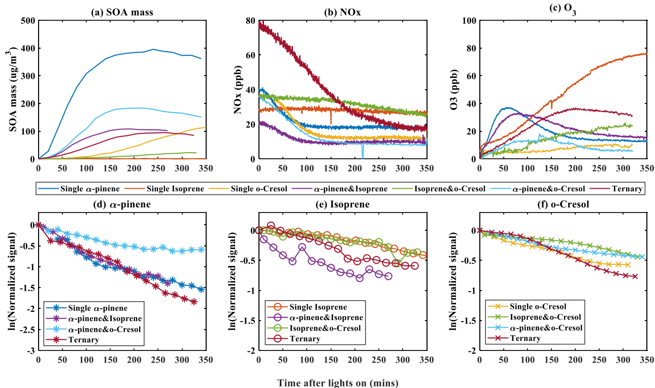
405 Figure 1: Evolution of gas and total SOA particle mass measurements during the photo-oxidation of VOCs after chamber illumination. (a) The SOA mass was measured using a high-resolution time-of-flight aerosol mass spectrometer (HR-ToF-AMS) during single, binary and ternary experiment. (b)–(c): Concentration of NO x and O 3 against time in all of single, binary and ternary experiments. (d)–(f): decay rate of VOC across all systems in. \alpha -pinene (b), isoprene(c) and o-cresol(d) in single, binary and ternary experiments respectively. 410
