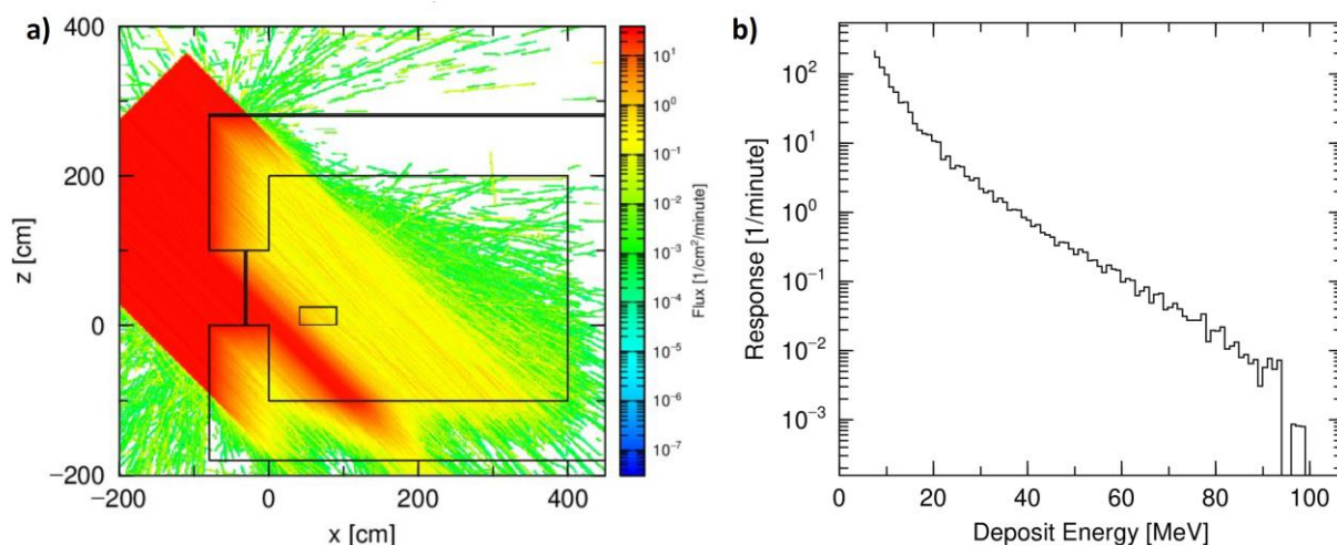
Figure 5: a) TGE source particles, the source is tilted by 45° from the vertical axis, and the energy spectra correspond observation by Chilingarian and Mailyan (2013). b) Deposit energy spectra inside the scintillator. Lower energy threshold was set to 6.5 MeV according to the setup of the detector.
