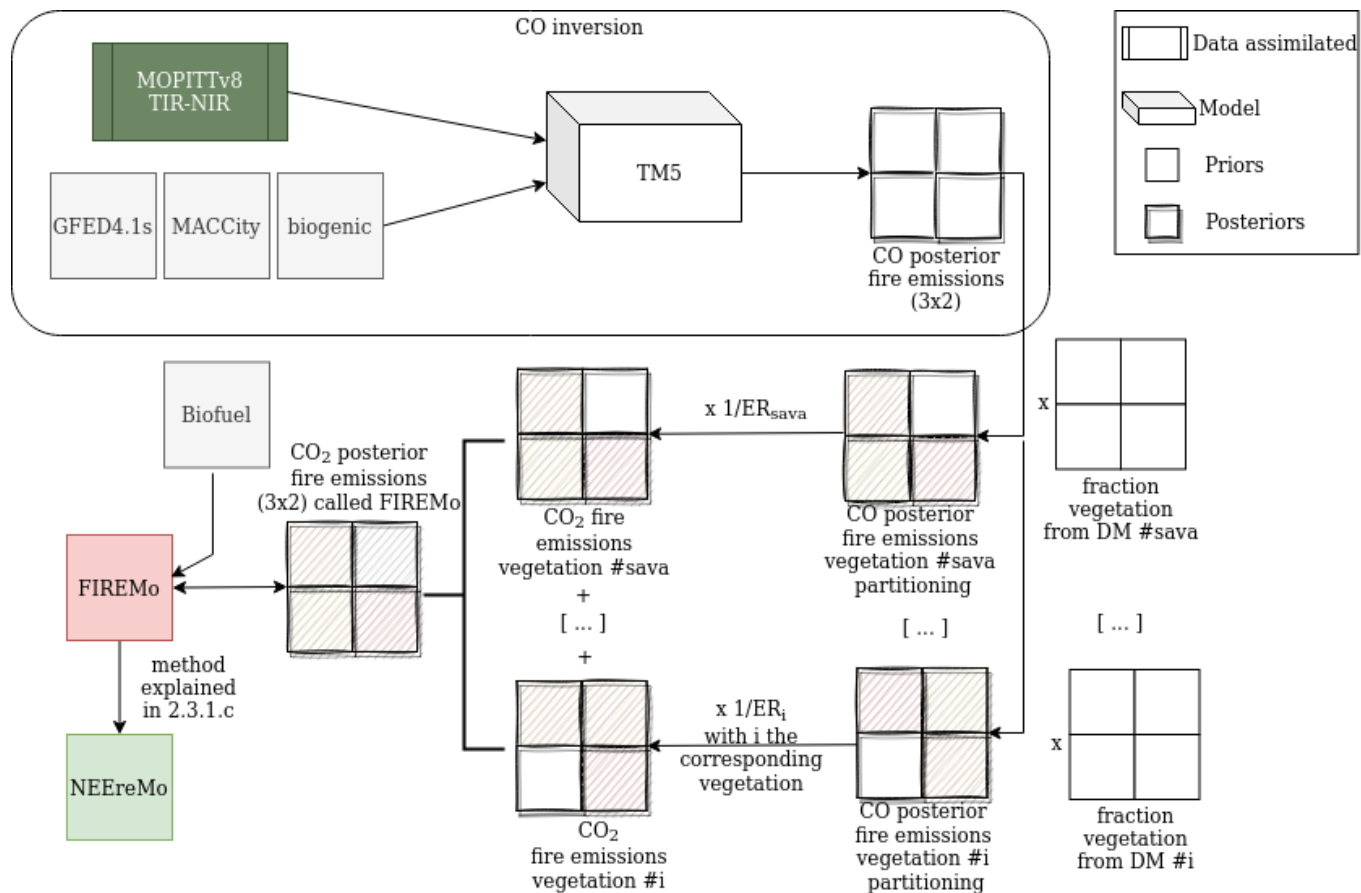
Figure 1. Flowchart of the FIREMO calculation from the CO inversion
