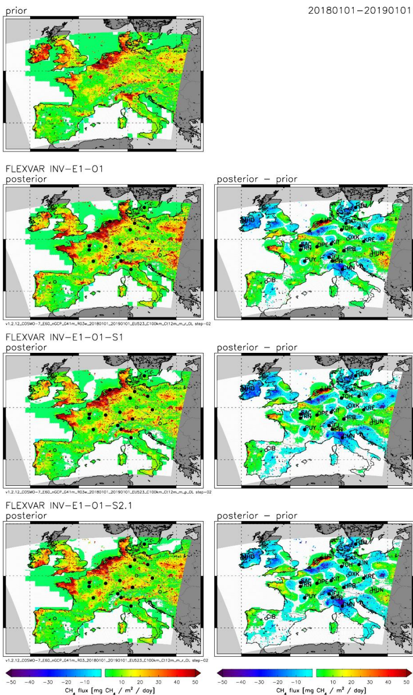
Figure 1: Sensitivity of FLEXVAR inversions to different approaches to calculate the baselines and to parameterize the model representation error. Upper left figure: prior emissions (emission data set E1). Second row: posterior emissions (left) and difference between posterior and prior emissions (right) for base inversion INV-E1-O1 (using the Rödenbeck baselines and the METEO model representation error). Third row: inversion INV-E1-O1-S1 using the particle position baselines. Fourth row: inversion INV-E1-O1-S2.1 using the OBS model representation error. All figures show annual average CH 4 emissions (or change in emissions, respectively) for 2018.
