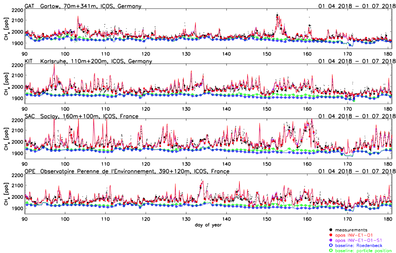
465 Figure 2: Time series of simulated and observed CH 4 mole fractions at stations GAT, KIT, SAC, and OPE for 3-month period from 01 April until 01 July 2018. Blue curve shows the Rödenbeck baselines, green the particle position baselines, red the posterior 470 CH 4 mole fractions for inversion INV-E1-O1 (using the Rödenbeck baselines), violet the posterior CH 4 mole fractions for inversion INV-E1-O1-S1 (using the particle position baselines) (owing to the similarity of both posterior simulations, however, the results of INV-E1-O1-S1 are largely overlaid by those of INV-E1-O1). Small black dots: hourly-averaged observations. Solid black circles: 475 assimilated observations. Coloured symbols show the corresponding assimilated values (solid circles: assimilated posterior mole fractions; open circles: baseline values used for the assimilation).
