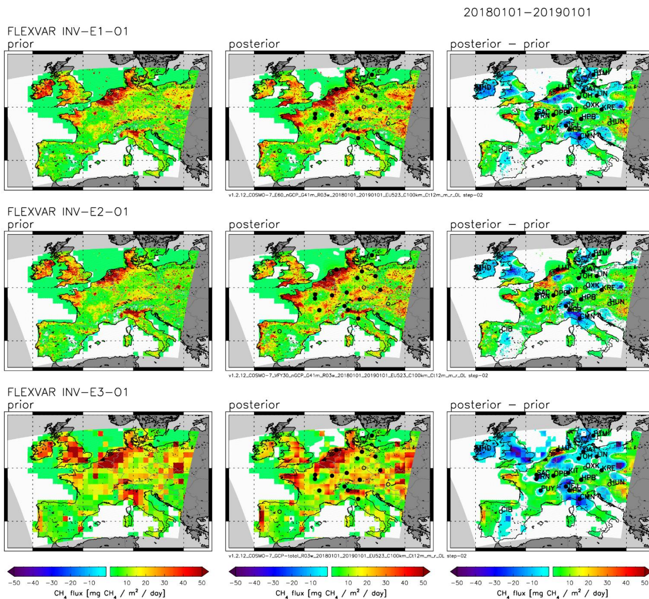
Figure 3: Sensitivity of FLEXVAR inversions to applied prior emission inventories. Upper row: inversion INV-E1-O1 using emission data set E1 as prior. Middle row: inversion INV-E2-O1 using emission data set E2 as prior. Lower row: inversion INV-E3-O1 using emission data set E3 as prior. Left column: prior emissions. Middle column: posterior emissions. Right column: difference between posterior and prior emissions. All figures show annual average \text{CH}_4 emissions (or change in emissions, respectively) for 2018.
