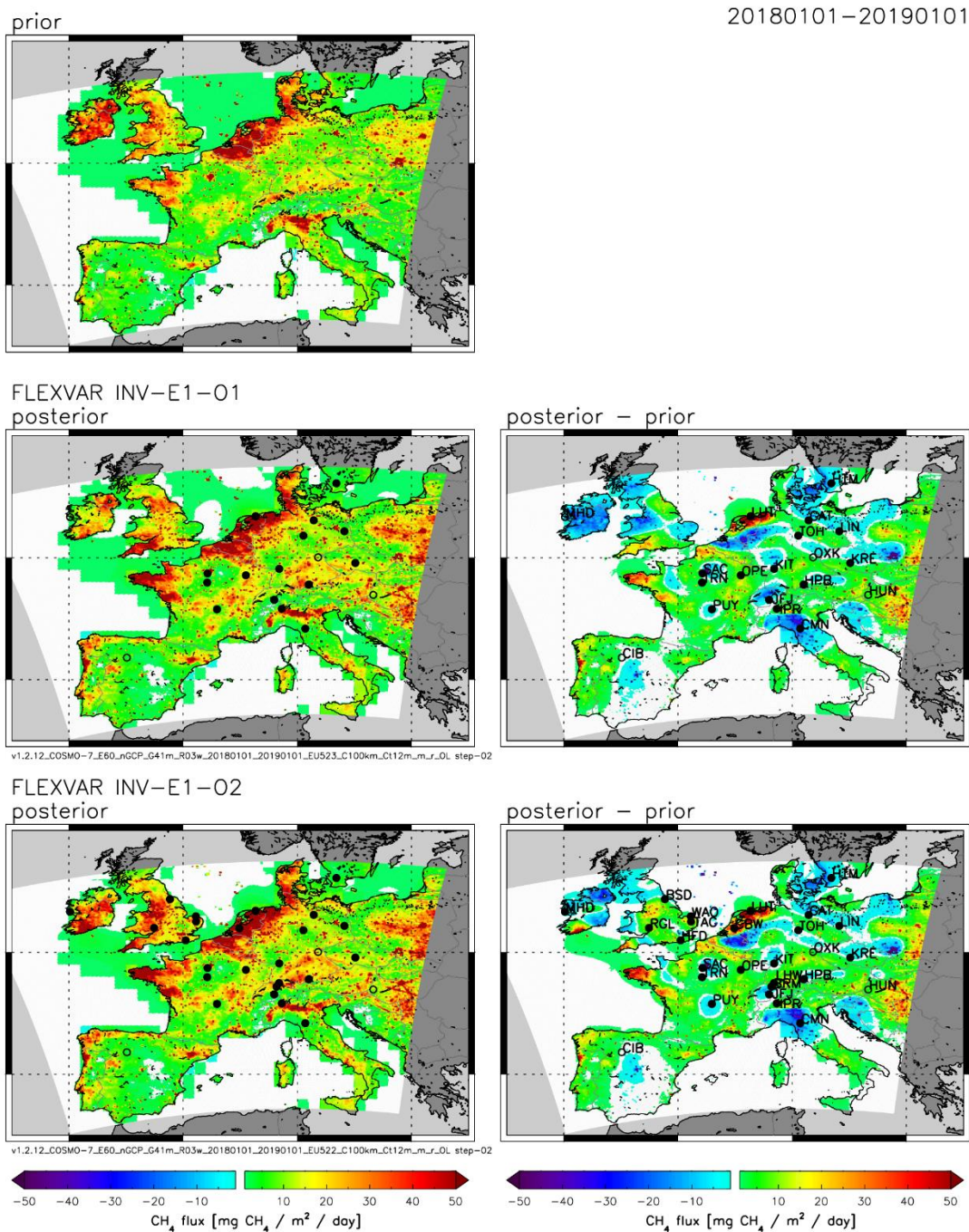
Figure 4: Sensitivity of FLEXVAR inversions to assimilated observations. Upper left figure: prior emission. Middle row: posterior emissions (left) and difference between posterior and prior emissions (right) for inversion INV-E1-O1 (using observation data set O1). Lower row: inversion INV-E1-O2 (using observation data set O2). Solid black circles show locations of stations with in situ data, open circles locations of stations with discrete air sampling. All figures show annual average CH 4 emissions (or change in emissions, respectively) for 2018.
