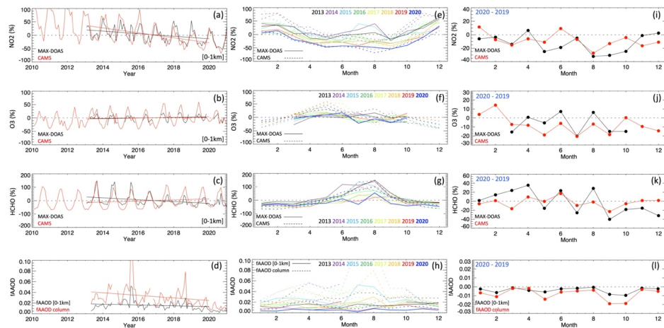
Figure 4: Left column: monthly time series of \text{NO}_2 (a), \text{O}_3 (b), and \text{HCHO} (c) partial column ( < 1 km) as recorded by the MAX-DOAS system and estimated by CAMS at Chiba University. Central column: seasonal monthly changes in MAX-DOAS observations and CAMS estimates of \text{NO}_2 (e), \text{O}_3 (f) and \text{HCHO} (g). Right column: differences (2020 minus 2019) in MAX-DOAS observations and CAMS estimates for \text{NO}_2 (i), \text{O}_3 (j) and \text{HCHO} (k). Results are shown as percentage changes with respect to the 2013–2019 average (left and central panels) and 2019 (right panel). Bottom panel: changes as described above but for fine mode light-absorbing aerosols i.e., fAAOD and fAAOD (0–1 km).
