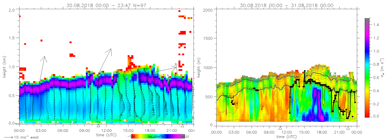
Figure A1. Example data from August 30, 2018. Left: Horizontal wind speed and direction (vectors) and attenuated backscatter ( \beta , color shading) as a function of time and height. Right: Standard deviation of vertical velocity from the wind lidar (color shading), backscatter ( \log_{10} \beta , thin gray lines), with \log_{10} \beta = -5 as a typical value for cloud base (thick gray line) and mixing layer height estimate (after Schween et al., 2014, thick black line with symbols). Note that the upper border of the region with backscatter is due to extinction of the laser signal and does not represent cloud top. Triangles at the abscissa indicate times of sunrise and sunset with night to the left and day on the left side.
