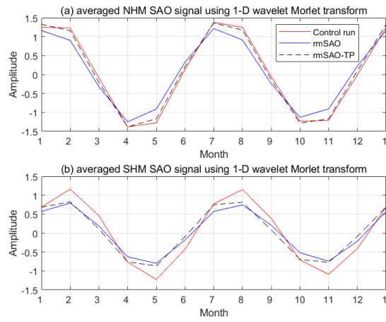
Figure 8. The average extracted SAO signals (5-7 months) based on 1-D wavelet Morlet transform for the Northern Hemisphere mid-latitudes (NHM) (a) and for the Southern Hemisphere mid-latitudes (SHM)(b). The red, blue and dashed black lines are results of the Control, rmSAO and rmSAO-TP runs, respectively.
