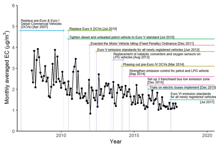
Figure 8. Ten-year variation of monthly EC concentration. The significant vehicular emission control measures implemented in Hong Kong are indicated in the top plot.
