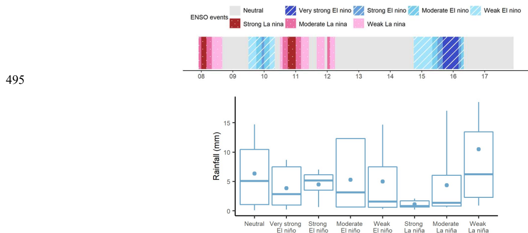
Figure 9. The temporal variation in strength of ENSO events in the 2008-2017 period (top), and the changes of rainfall (bottom) under different strength levels of ENSO events.
