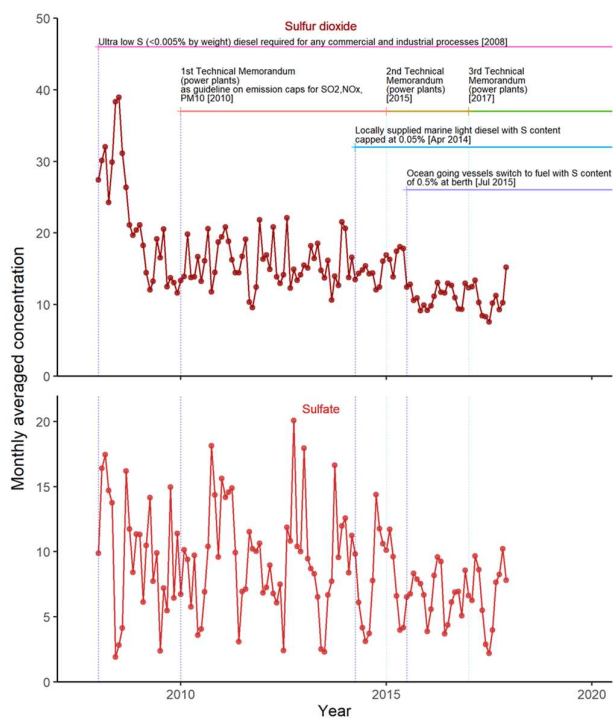
380 Figure 7. Ten-year variation of monthly SO 2 and sulfate concentration. The significant SO 2 emission control measures implemented in Hong Kong are indicated in the top plot. The unit of concentration is µg m -3 .
