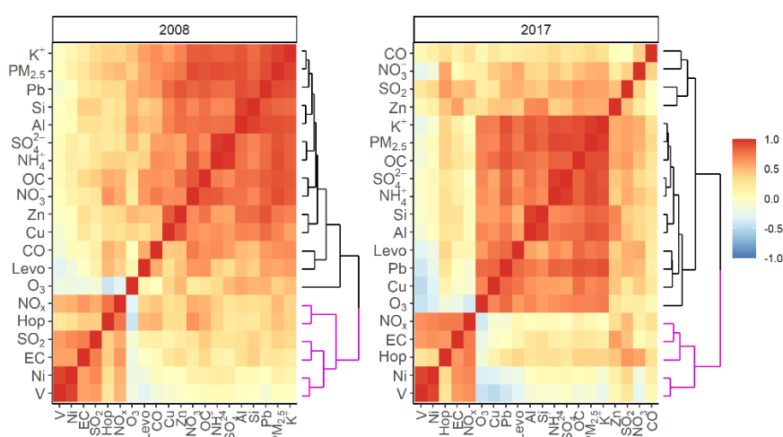
315 Figure 5. Correlation matrix of gaseous and particulate pollutants with hierarchical clustering results at 2008 (left) and at 2017 (right). Clusters: pink – local sources; black – regional sources.
