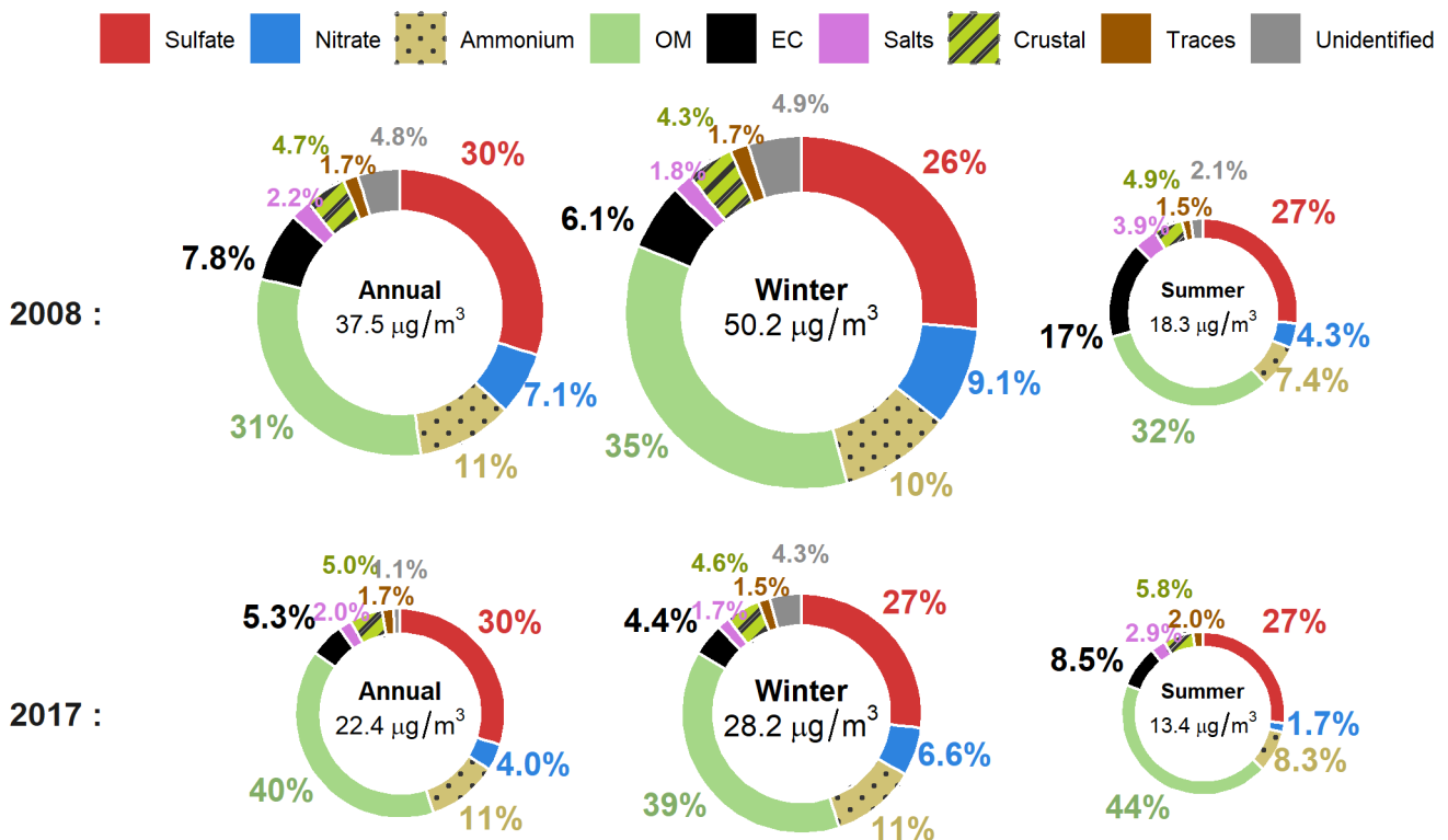
245 Figure 3. Comparison of average PM_{2.5} compositions between the starting year (2008) and the ending year (2017) of the decade. In each year, three averages are shown, corresponding to annual, winter, and summer, and the donut size is proportional to the PM_{2.5} concentration.
