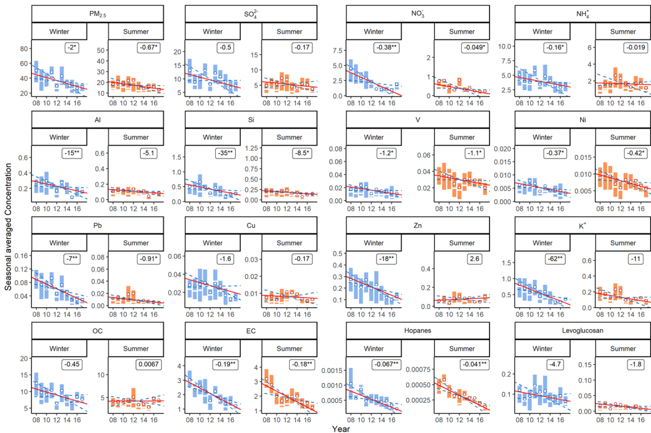
Figure 6. Ten-year variations of seasonal average concentrations of PM 2.5 and select components for the winter (blue) and summer (orange) from 2008 to 2017. Red lines indicate the Sen's slope, blue dashed lines indicate the 95% confidence intervals.
