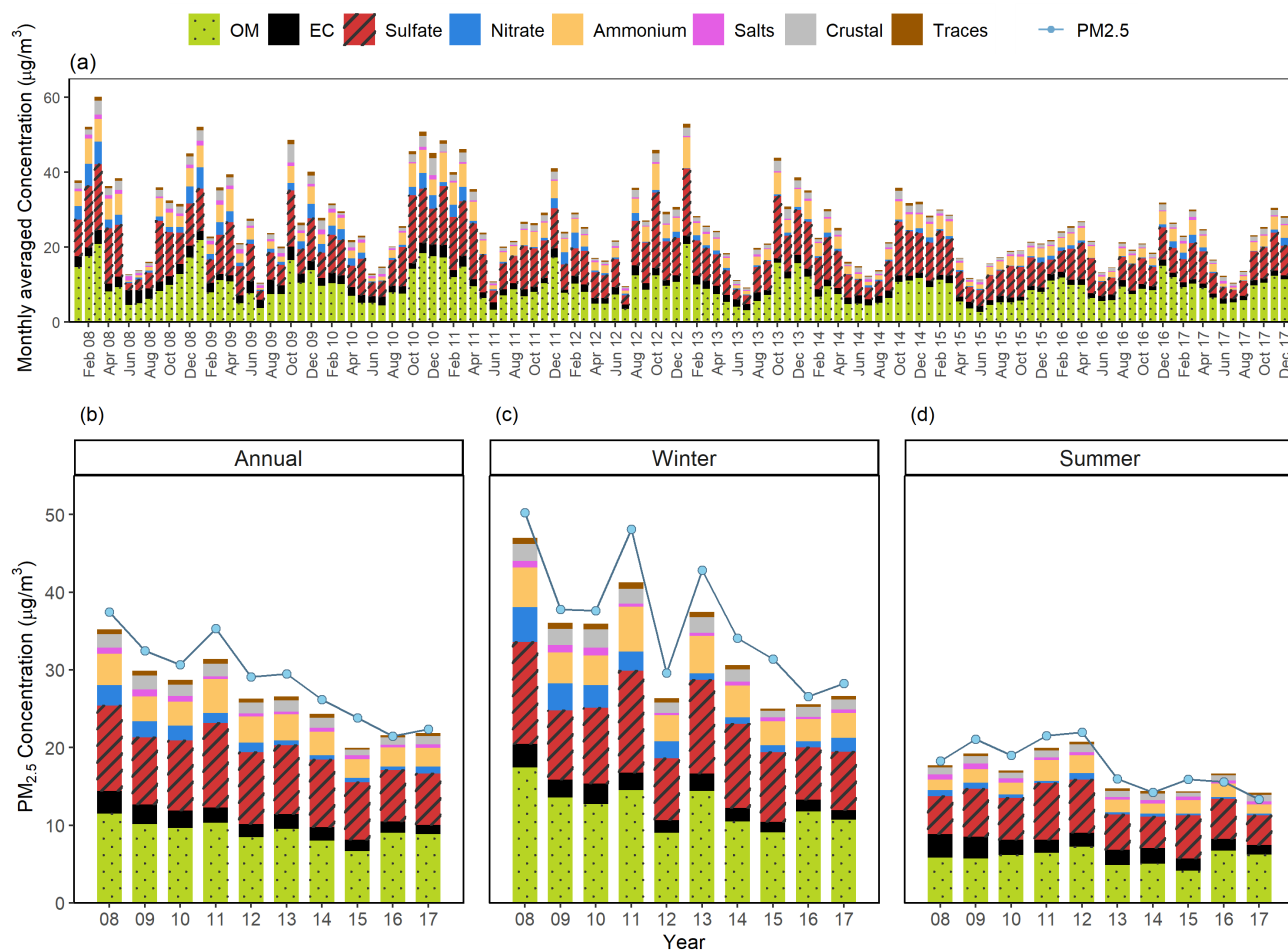
230 Figure 2. Time series of PM 2.5 chemical composition from 2008 to 2017 in the form of (a) monthly averages, (b) annual average, (c) winter seasonal averages, and (d) summer seasonal averages. In the legends, “Salts” includes Na + and Cl - ; “Crustal” represents crustal materials,
