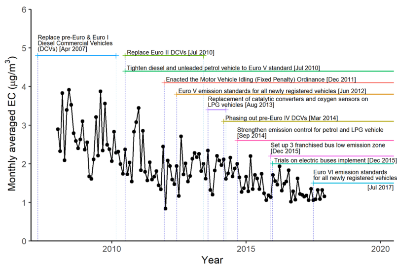
415 Figure 8. Ten-year variation of monthly EC concentration. The significant vehicular emission control measures implemented in Hong Kong are indicated in the top plot.
