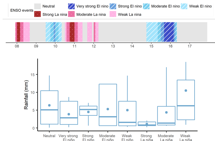
Figure 9. The temporal variation in strength of ENSO events in 2008-2017 period (top), and the changes of rainfall (bottom) under different strength levels of ENSO events.
