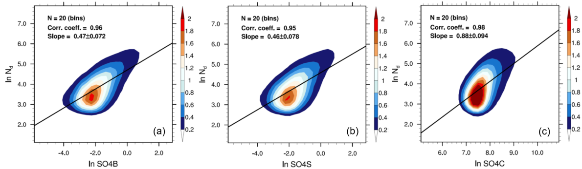
Figure 7. Two-dimensional probability density functions of \ln N_d versus (a) \ln \text{SO4B} , (b) \ln \text{SO4S} , and (c) \ln \text{SO4C} , respectively, for the period 2006–2009. Sample numbers ( N ), correlation coefficients, and regression slopes with 95 % uncertainty estimates (according to Student’s t-test) for pre-binned \text{SO4} - N_d pairs are displayed in the upper left of each plot.
