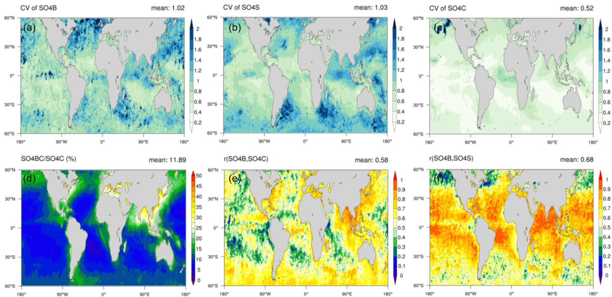
Figure 8. Map of coefficients of variations (CV) of (a) \text{SO4B} , (b) \text{SO4S} , and (c) \text{SO4C} , (d) ratio of column mass of \text{SO4} below clouds ( \text{SO4BC} ) to \text{SO4C} (%), Pearson’s correlation coefficients of \text{SO4B} with (e) \text{SO4C} and (f) \text{SO4S} , which are calculated for each 1^\circ \times 1^\circ grid box over the period 2006–2009.
