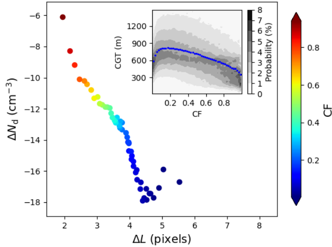
Figure 6. Relationships between \Delta L and \Delta N_d , where the data are grouped as a function of CF with each CF bin containing same number of samples. Joint histogram between CF and CGT is shown in the inner plot, where the blue dot shows the median CGT at each CF bin.
