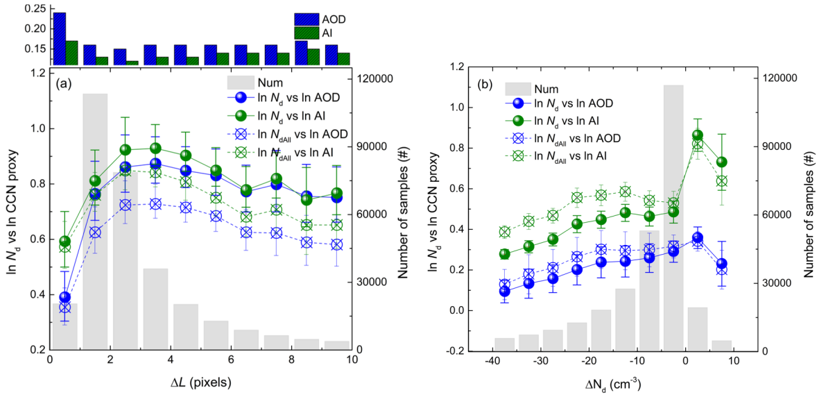
Figure 5. Dependence of the linear regression slopes of \ln N_d ( \ln N_{dAll} ) versus \ln AOD ( \ln AI ) on (a) \Delta L and (b) \Delta N_d derived via the pre-binned approach. Data are grouped into 10 fixed \Delta L ( \Delta N_d ) intervals for the calculation of slopes. Error bars indicate the 95 % confidence interval of the linear regression, and the gray bars denote the total number of samples for each bin. The change of AOD (AI) with \Delta L is also shown in the panel (a). The equivalent Fig. S3 shows similar results based on the all-data approach.
