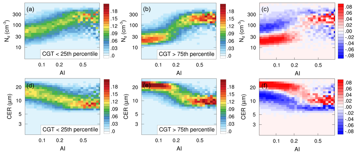
Figure 3. Joint histograms between AI and N_d (CER) created for weak and strong updraft conditions, as defined by the lowest and the highest CGT quartiles, respectively. The difference plots between strong and weak cases are shown at the end of each row. The histograms are normalized so each column sums to 1, such that the histograms show the probability of observing a specific N_d (CER), given a certain AI.
