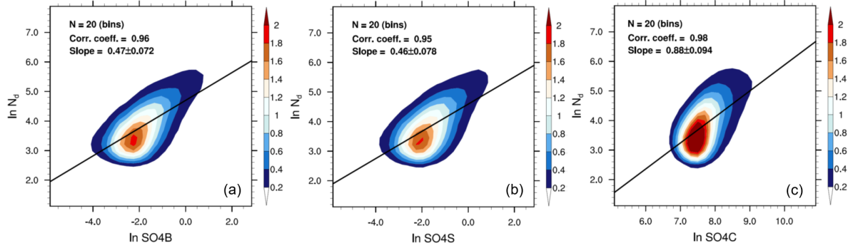
Figure 7. Two-dimensional probability density functions of \ln N_d versus (a) \ln SO_{4B} , (b) \ln SO_{4S} , and (c) \ln SO_{4C} , respectively, for the period 2006–2009. Sample numbers ( N ), correlation coefficients, and regression slopes with 95 % uncertainty estimates (according to Student’s t-test) for pre-binned SO_4 - N_d pairs are displayed in the upper left of each plot.
