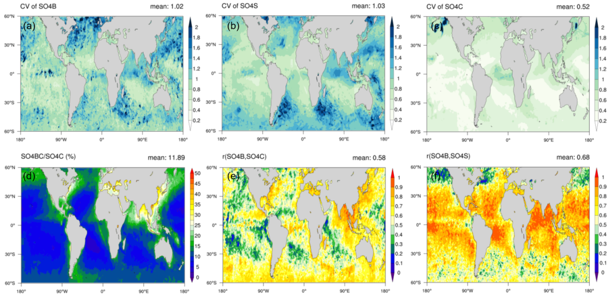
Figure 8. Map of coefficients of variations (CV) of (a) SO_{4B} , (b) SO_{4S} , and (c) SO_{4C} , (d) ratio of column mass of SO_4 below clouds ( SO_{4BC} ) to SO_{4C} (%), Pearson’s correlation coefficients of SO_{4B} with (e) SO_{4C} and (f) SO_{4S} , which are calculated for each 1^\circ \times 1^\circ grid box over the period 2006–2009.
