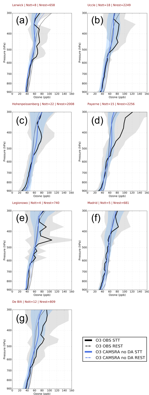
Figure 8. Vertical profiles of observed (black) and CAMSRA no DA (blue) ozone concentrations (ppb) during STT events (thick solid line) as well as during the rest of events (thin dashed line) at the WOUDC ozonesonde stations of a) Lerwick (UK), b) Uccle (Belgium), c) Hehenpeissenberg (Germany), d) Payerne (Switzerland), e) Legionowo (Poland), (f) Madrid (Spain), and (g) De Bilt (the Netherlands). The grey and sandybrown shaded areas depict the \pm one standard deviation of ozone vertical profiles during STT events in observations and CAMSRA no DA, respectively.
