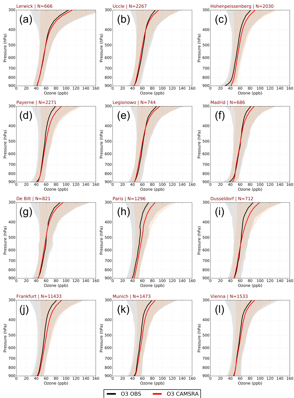
Figure 3. Vertical profiles of observed (black) and CAMSRA (red) ozone concentrations (ppb) at the WOUDC ozonesonde stations of a) Lerwick (UK), b) Uccle (Belgium), c) Hehenpeissenberg (Germany), d) Payerne (Switzerland), e) Legionowo (Poland), f) Madrid (Spain), and (g) De Bilt (the Netherlands); at the IAGOS airports of h) Paris (France), i) Düsseldorf (Germany), j) Frankfurt (Germany), k) Munich (Germany), and l) Vienna (Austria) for the period 2003–2018. The grey and sandybrown shaded areas depict the \pm one standard deviation of ozone vertical profiles in observations and CAMSRA, respectively.
