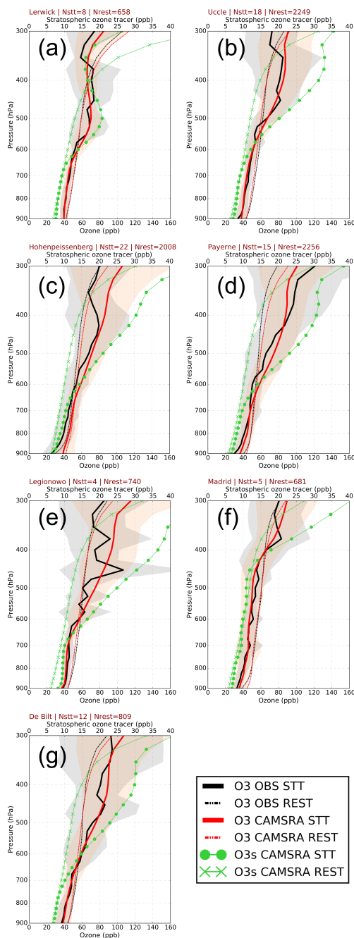
Figure 4. Vertical profiles of observed (black) and CAMSRA (red) ozone concentrations (ppb) during STT events (thick solid line) as well as during the rest of events (thin dashed line) at the WOUDC ozonesonde stations of a) Lerwick (UK), b) Uccle (Belgium), c) Hohenpeissenberg (Germany), d) Payerne (Switzerland), e) Legionowo (Poland), (f) Madrid (Spain), and (g) De Bilt (the Netherlands). Also shown are the vertical profiles of stratospheric ozone tracer concentrations (ppb) during STT (green circles) and rest of events (green x markers). The grey and sandybrown shaded areas depict the \pm one standard deviation of ozone vertical profiles during STT events in observations and CAMSRA, respectively. Keep in mind that O_3 and O_{3s} concentrations are presented in different horizontal axes.
