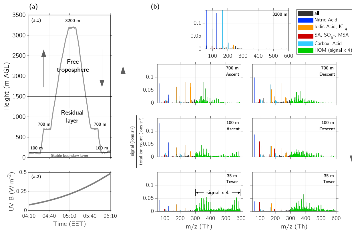
Figure 6. Vertical profile of ions above Hyttiälä on 2 May 2017 04:00–06:00 EET. (a.1) Height profile of the flight measurements and indication of the different layers (stable boundary layer (SBL), residual layer (RL), and free troposphere (FT)). (a.2) UV-B radiation measured on the ground at SMEAR II station during the flight. (b) Mass spectra measured with API-TOF at different heights. The altitude where the mass spectra were measured is indicated in the figures and can be compared with the height profile of panel (a). The lowest mass spectra show the measurements from the tower at SMEAR II station at 35 m height, while the presented data is covering the time period of the lowest level measurements at 100 m (04:10–04:20 EET and 05:55–06:05 EET) to be comparable. The signal of the HOM dominated ions (green) between 300–600 Th is multiplied by factor 4 to make the pattern more visible. A peak list of the different layers can be found in Table A1. The colour code shows the composition of the compounds: nitric acid (blue), iodic acid and iodine-chlorine (yellow), sulfuric acid (SA), \text{SO}_5^- and MSA (red), carboxylic acids (cyan), and HOM dominated ions (green).
