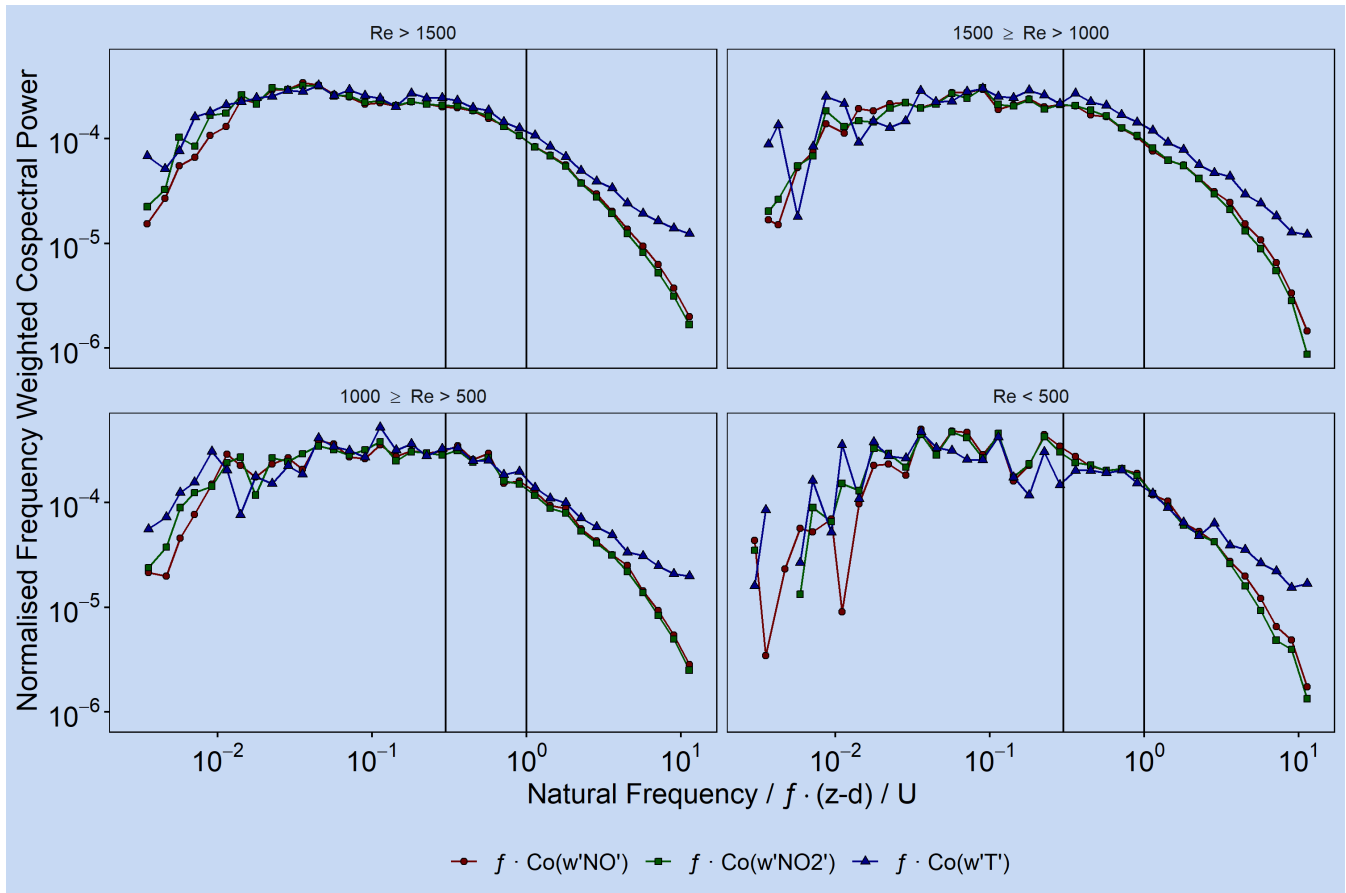
Figure 6. Normalised co-spectra of vertical wind with NO (red, circle), NO 2 (green, square) and temperature (dark blue, triangle). Co-spectra are grouped by main sample line Reynolds number. Vertical bars mark 0.3 Hz and 1 Hz where data at frequencies greater than these have been used to derive the correction factors presented in table 1
