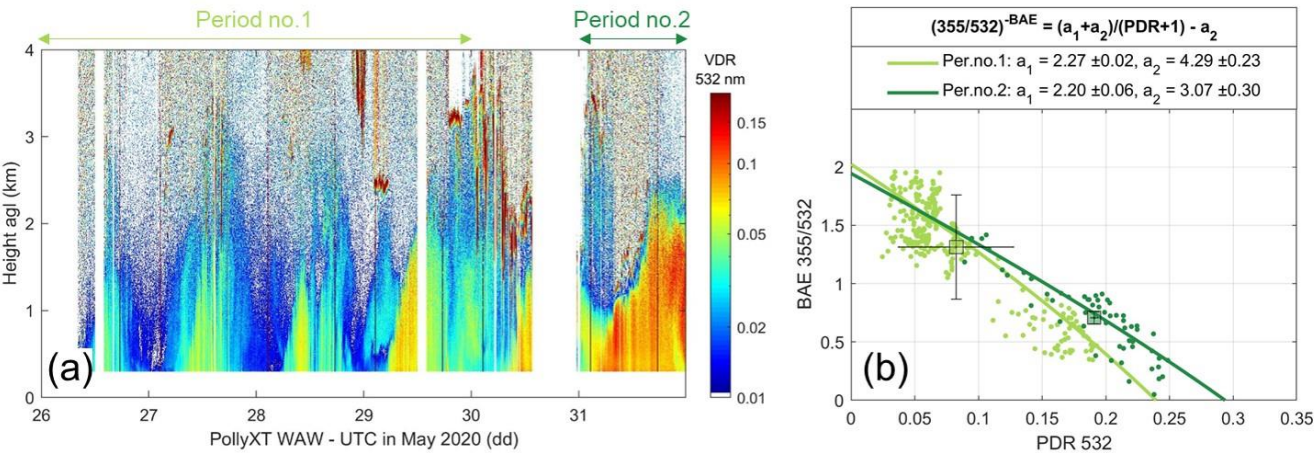
Figure 4. (a) Time–height cross section of volume depolarization ratio (VDR) at 532 nm from Polly XT at Warsaw station on 26–31 May 2020. Selected two periods are indicated on the top. (b) Similar as Fig. 2, but for two periods at Warsaw station.
