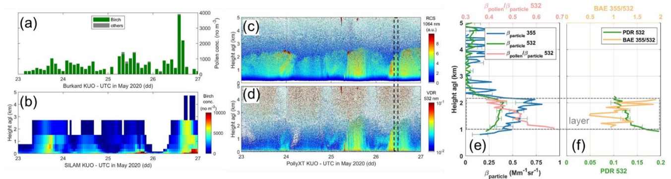
Figure 3. Overview of the pollen period and a case example at Kuopio station. (a) Pollen concentrations from Burkard sampler at the roof level. (b) Birch pollen concentrations from SILAM model. Time–height cross section of (c) range-corrected signal (RCS) at 1064 nm and (d) Volume depolarization ratio (VDR) at 532 nm of Polly XT . Vertical profiles of (e) backscatter coefficients, and the
