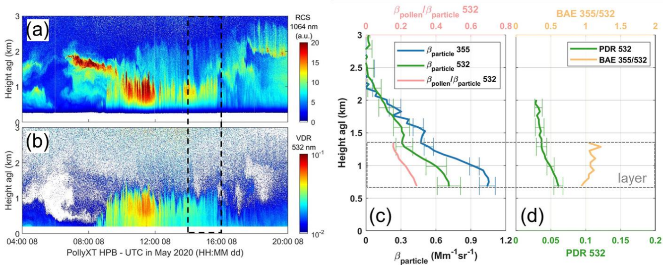
340 Figure 5. Case example in period no.1 of Hohenpeißenberg station. Time–height cross section of (a) range-corrected signal (RCS) at 1064 nm and (b) volume depolarization ratio (VDR) at 532 nm from Polly XT . Vertical profiles of (c) backscatter coefficients, and the pollen backscatter contribution, (d) backscatter-related Ångström exponent (BAE) and the particle linear depolarization ratio (PDR), of the selected time period (black dashed box in a,b). Selected layer is shown in grey dashed box.
