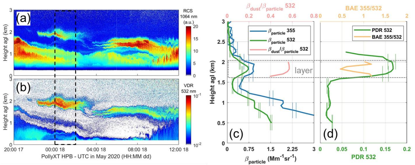
345 Figure 6. Similar as Fig. 5, but in period no.2 of Hohenpeißenberg station.
