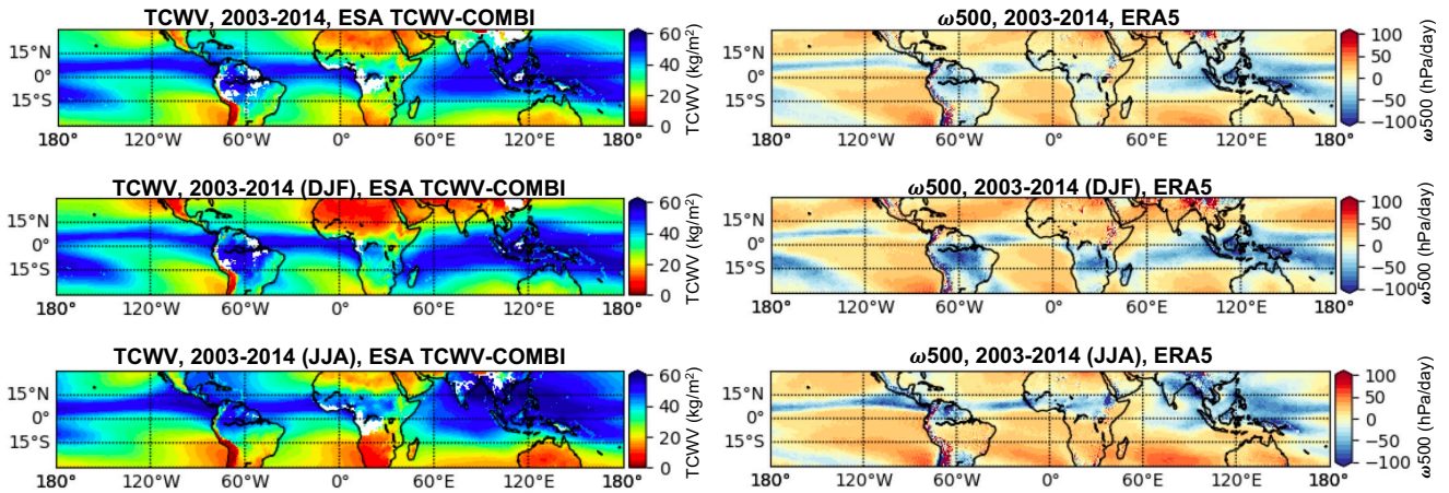
Figure 2. Maps of the TCWV-COMBI (in kg/m 2 ) during 2003 - 2014 for the tropical region (30°S - 30°N) for the whole period, Winter (December, January and February - DJF), and Summer (June, July, and August - JJA) and the corresponding maps of ERA5 \omega_{500} (in hPa/day).
