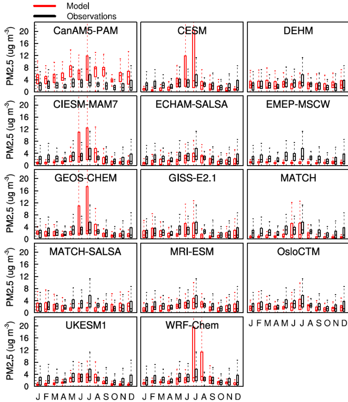
Fig S3. Modelled and measured monthly mean surface PM 2.5 concentrations in the Arctic for 2014-15.
