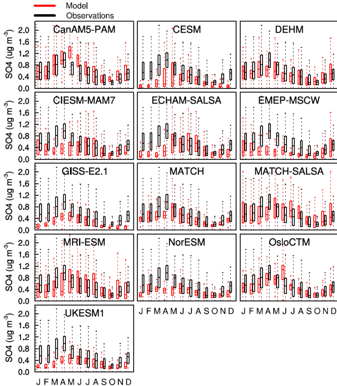
Fig S1: Measured (black) and modelled (red) \text{SO}_4^{2-} seasonal cycle, where box and whiskers represent the range from all Arctic sites grouped together for 2008-9.
