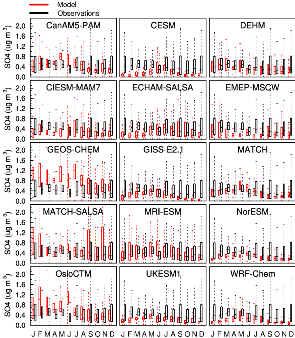
Fig S2. Measured (black) and modelled (red) \text{SO}_4^{2-} seasonal cycle, where box and whiskers represent the range from all Arctic sites grouped together for 2014-15.
