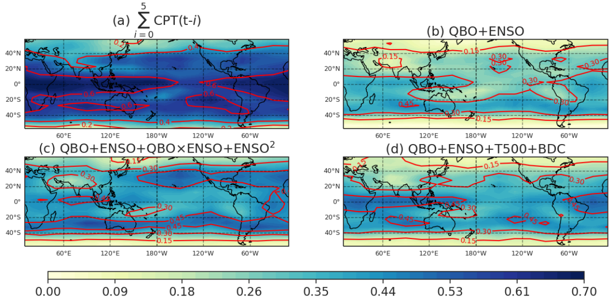
Figure 3. The R^2 of the MLR between water vapor anomalies at the 82.54 hPa level with the four groups of predictors: (a) cold point temperatures; (b) QBO and ENSO; (c) as in (b) but adding in \text{ENSO}^2 and \text{QBO} \times \text{ENSO} ; (d) as in (b) but adding in T500hPa and the BDC. This MLR spans from 2005 to 2019 and uses the 3D SWOOSH product. The regression is reconstructed directly from all predictors, i.e., in-sample.
