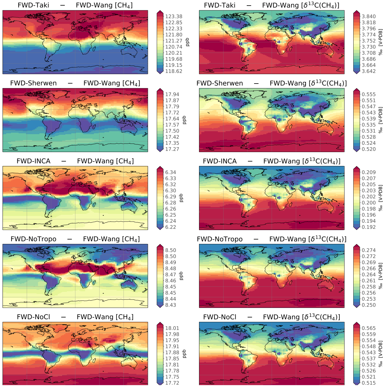
Figure 2. Surface absolute bias between FWD-* and FWD-Wang simulations averaged over 2010-2018. Temporal average-averaging is performed before subtraction. First-Left column displays the biases between CH 4 mole fractions. Second-Right column shows the biases between \delta^{13}\text{C}(\text{CH}_4) values. Note that the scales are different for each panel.
