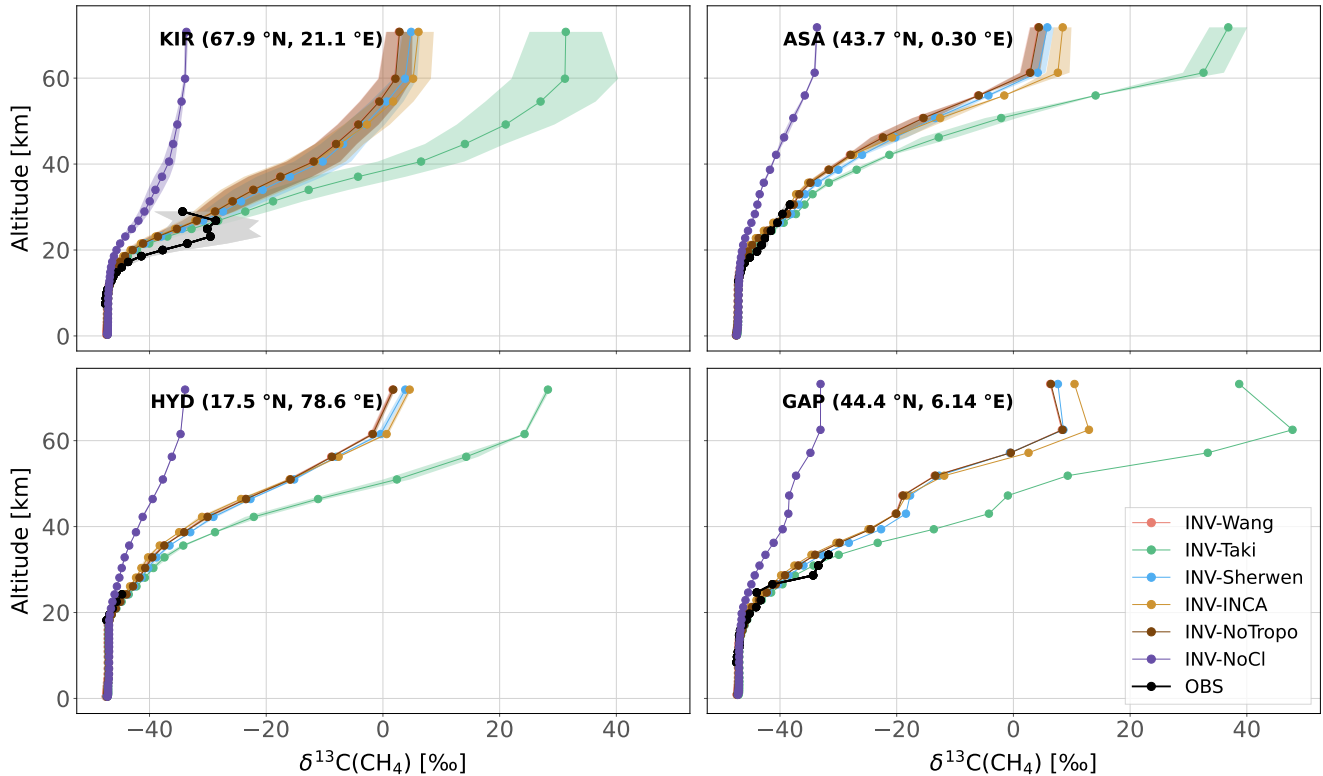
Figure 5. Observed and simulated \delta^{13}\text{C}(\text{CH}_4) vertical profiles for four locations. All available vertical profiles in each region have been averaged. Shaded areas indicate the standard deviations of this average. Note that measurement uncertainties (around 0.2 ‰) are much lower than the x-axis range. KIR : Kiruna, Sweden (67.9 °N, 21.10 °E) ; ASA : Aire sur l’Adour, France (43.70 °N, 0.30 °E) ; HYD : Hyderabad, India (17.5 °N, 78.60 °E) ; GAP : Gap, France (44.44 °N, 6.14 °E).
