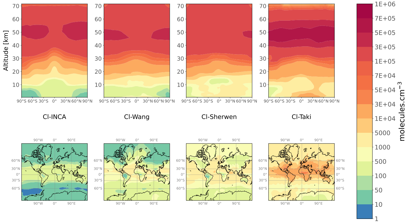
Figure 1. Annual mean meridional cross-section (upper panels) and tropospheric CI concentrations (lower panels) for the four 3-D fields CI-INCA, CI-Wang, CI-Sherwen and CI-Taki.
