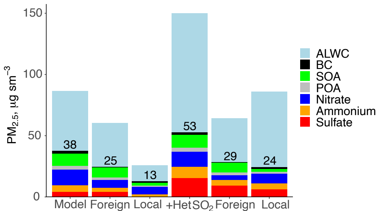
Figure 1314. Composition of model PM 2.5 during the Transport/Haze period. The foreign and local contributions and model sensitivity test including heterogeneous uptake of SO 2 to aerosol (Het SO 2 ) are calculated as discussed in Section 6. The total PM 2.5 excluding aerosol liquid water content (ALWC) is given for each simulation.
