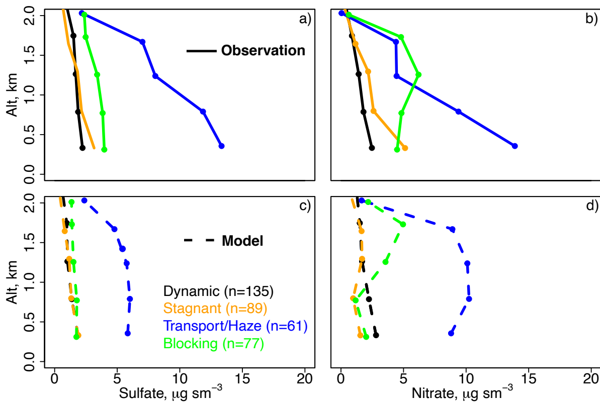
55 Figure 3. Mean vertical profiles of a) observed sulfate, b) observed nitrate, c) model sulfate, and d) model nitrate for the descents over Olympic Park for each meteorological period. The observations (solid lines) and model (dashed lines) are binned to the nearest 0.5 km below 2 km.
