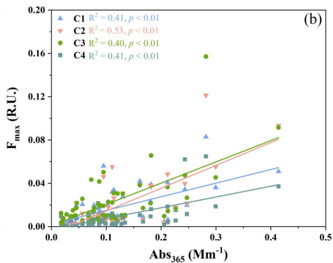
Fig. 5. The EEMs components in PM 2.5 (P1-P2) and cloud water (C1-C4) that were identified by PARAFAC model, and the correlation between each chromophore F_{\max} and Abs_{365} in (a) PM 2.5 , and (b) cloud water.
