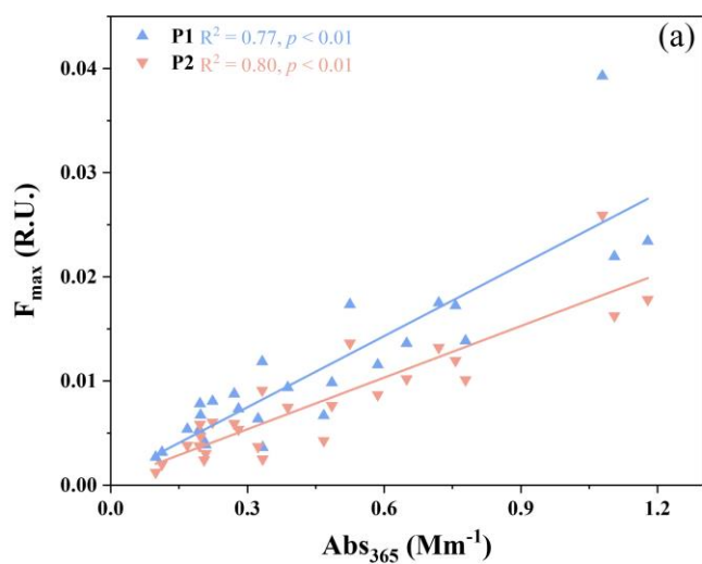
Fig. 5. The EEMs components in PM 2.5 (P1-P2) and cloud water (C1-C4) that were identified by PARAFAC model, and the correlation between each chromophore F_{\max} and Abs_{365} in (a) PM 2.5 , and (b) cloud water.
