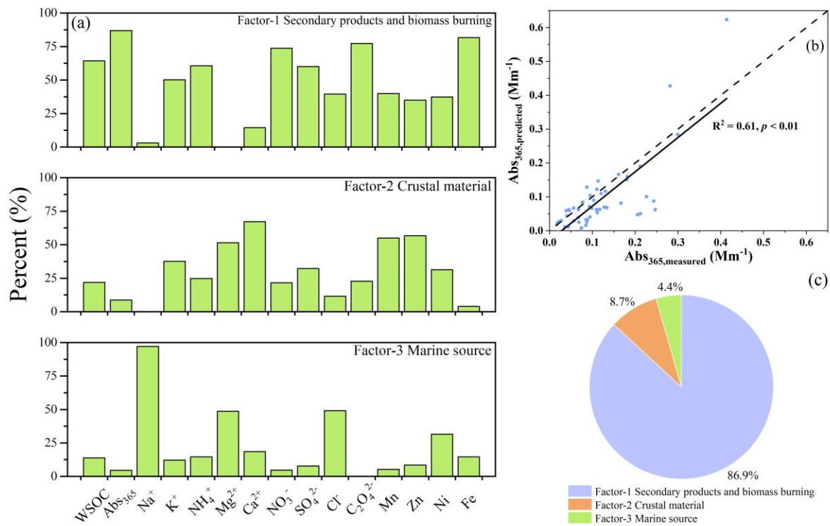
Fig. 4. (a) The composition profiles (% of each species) for the three factors simulated of cloud water by PMF, and (b) the correlation of measured, and predicted Abs 365 , and (c) the source apportionment for Abs 365 in cloud water.
