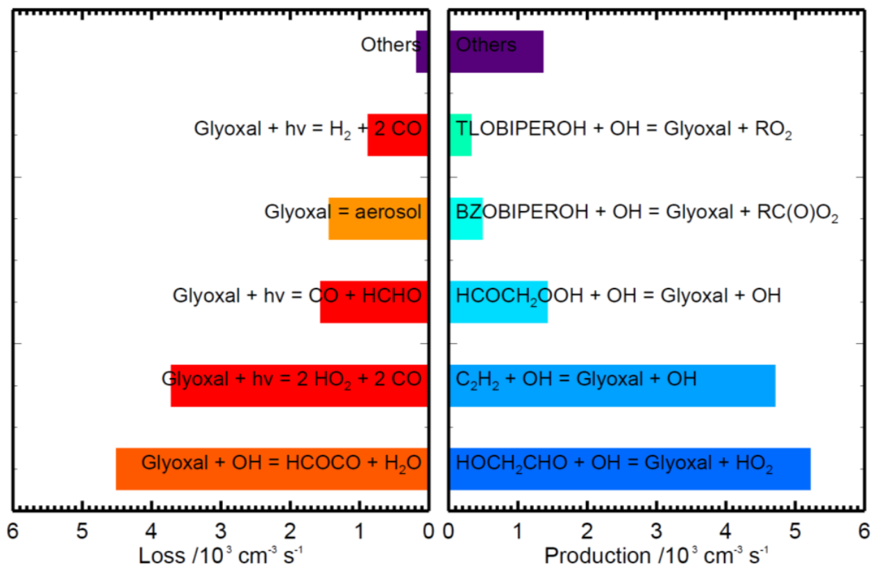
2 Figure 11: Midday (1100-1300 hours) average glyoxal budgets for the base model run for both measurement periods 4 combined. Chemical names are as given by the MCM. Note that there are three photolysis channels contributing to 6 the loss of glyoxal which are shown separately but constitute the dominant loss process overall. For information on molecular formulae and details of production mechanisms of BZOBIPEROH and TLOBIPEROH, please see: http://mcm.york.ac.uk/roots.htm#aromatics .
