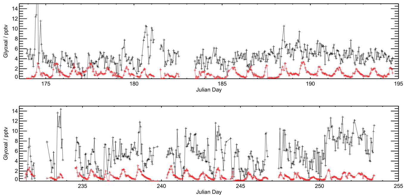
Figure 7: Time series of observed (black) and modelled (red) glyoxal during ORC 3 . Data are shown for model output every 60 min. The upper panel shows data from the first measurement campaign (Julian days 173 to 195), with the lower panel showing data from the second measurement campaign (Julian days 230 to 255).
