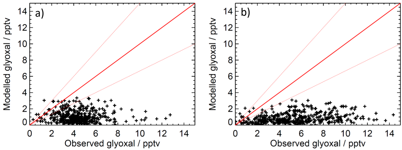
Figure 8: Modelled vs observed glyoxal for (a) the first measurement period and (b) the second measurement period
