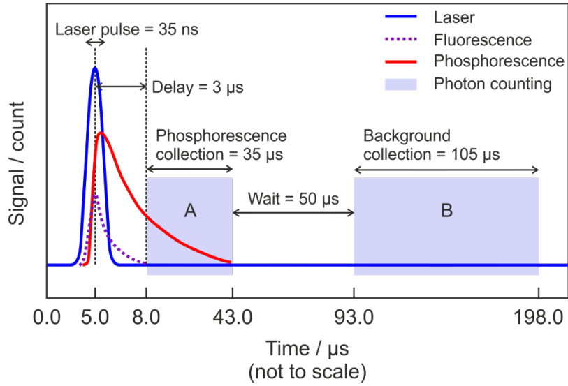
4 Figure 2: Schematic diagram showing the timing scheme for signal acquisition. The start of the cycle (time = 0.0 \mu\text{s} ) is 5 defined by the laser trigger. Blue = Ti:Sapphire laser pulse at \lambda \sim 440 \text{ nm} ; dashed purple = short-lived fluorescence 6 from the cell anodising dye, optics, and interfering species (e.g. \text{NO}_2 ); red = glyoxal phosphorescence; light (not to 7 scale) blue shading = photon counting. Region A indicates the gate for measurement of the combined 8 phosphorescence signal, remaining laser scattered light signal and background signal, while region B indicates and the 9 gate for measurement of the background signal alone.
