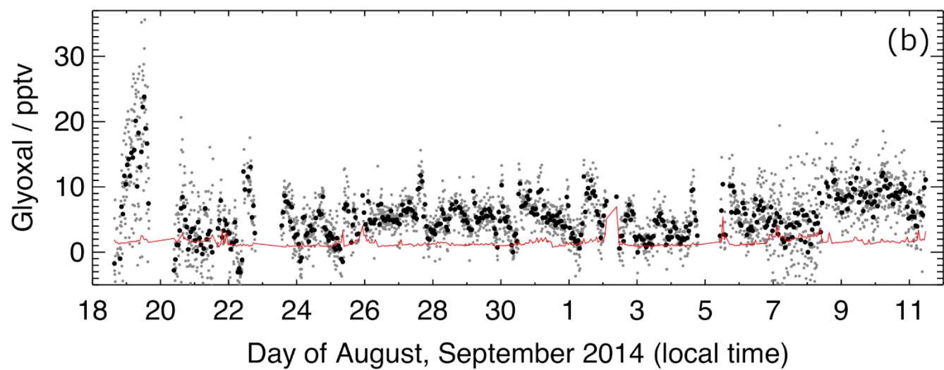
4 Figure 5: Time series of glyoxal data during (a) campaign 1 and (b) campaign 2. Black data points show 1-hour mean; 6 grey data points show the mean for a single measurement cycle (approximately 7 minute); red line shows limit of 8 detection.
