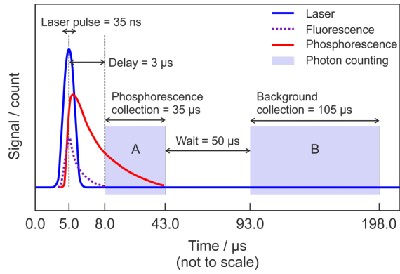
4 Figure 2: Schematic diagram showing the timing scheme for signal acquisition. The start of the cycle (time = 0.0 \mu s) is 6 defined by the laser trigger. Blue = Ti:Sapphire laser pulse at \lambda \sim 440 nm; dashed purple = short-lived fluorescence 8 from the cell anodising dye, optics, and interfering species (e.g. \text{NO}_2 ); red = glyoxal phosphorescence; light (not to scale) blue shading = photon counting. Region A indicates the gate for measurement of the combined phosphorescence signal, remaining laser scattered light signal and background signal, while region B indicates and the gate for measurement of the background signal alone.
