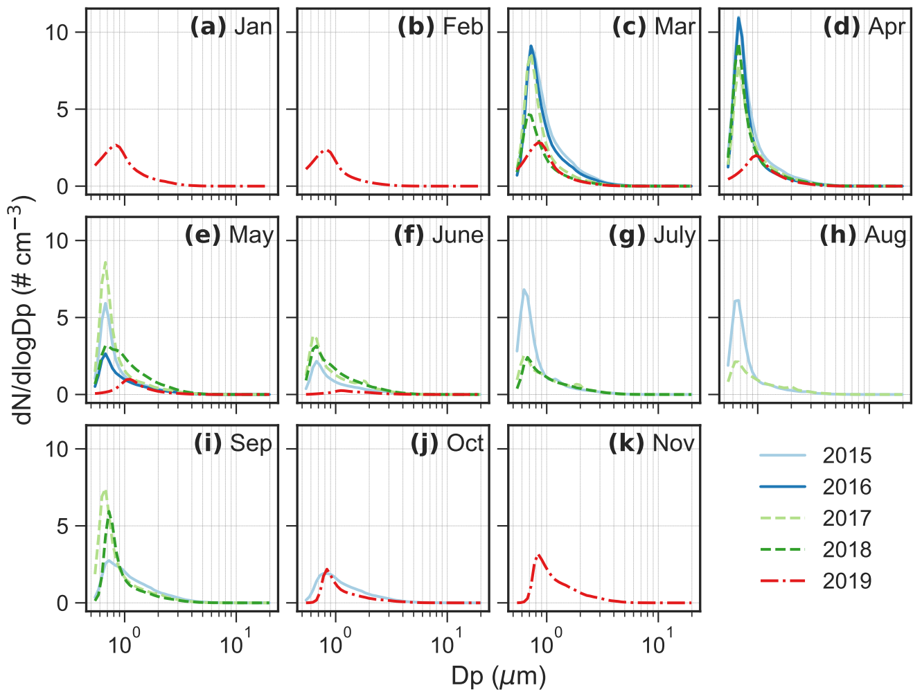
Figure A1. Monthly average aerosol number size distribution from 2015 to 2019. Missing data in some months but good data coverage from March to June. No data available in December.
