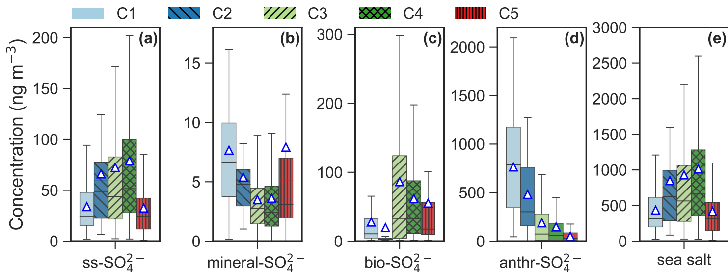
Figure 7. Box plot of (a) sea-salt SO 4 2- (ss-SO 4 2- ), (b) mineral SO 4 2- (mineral-SO 4 2- ), (c) biogenic SO 4 2- (bio-SO 4 2- ), (d) anthropogenic SO 4 2- (anthr-SO 4 2- ) and (e) sea salt for each cluster. The (e) sea salt aerosol is calculated by multiplying the ss-Na + by a factor of 3.248 (Kerminen et al., 2000; Brewer, 1975). The mean values are marked as triangles.
