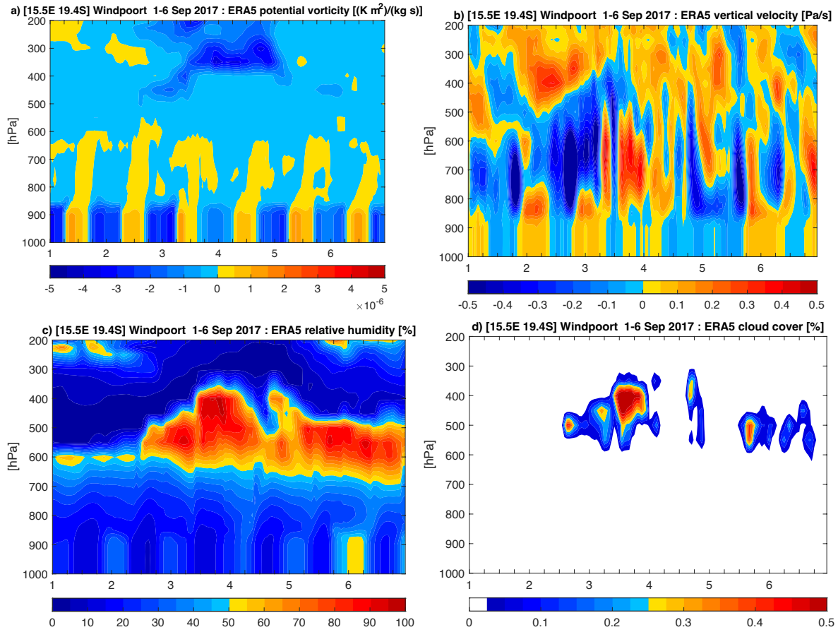
Figure 13. Time-height cross-section of (a) potential vorticity ( K\ m^2\ kg^{-1}\ s^{-1} ), (b) vertical velocity ( Pa\ s^{-1} ), (c) relative humidity (%) and (d) cloud cover over Windpoort between 1 and 6 September 2017 from hourly ERA 5 reanalysis. Ascending motions are associated with negative \omega values.
