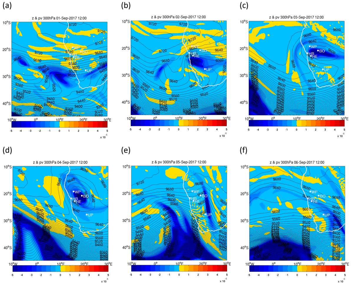
Figure 3: Geopotential (m, contours) and potential vorticity ( \text{K m}^2 \text{kg}^{-1} \text{s}^{-1} , colour) at 300 hPa at 1200 UTC on (a) 1 September , (b) 2 September , (c) 3 September , (d) 4 September , (e) 5 September and (f) 6 September 2017, from ERA 5 reanalysis. The names of the instrumented sites appear in white (from north to south): WP is Windpoort, BO is Bonanza, HB is Henties Bay, HE is HESS (Namibia) and UP is Uptington (South Africa).
