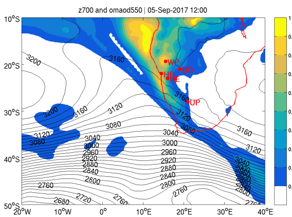
Figure 4: Geopotential at 700 hPa (contours) and organic matter AOT (colour) at 1200 UTC on (a) 3 September, (b) 4 September, (c) 5 September and (d) 6 September 2017, from CAMS reanalysis. The names of the instrumented sites appear in red (from north to south): WP is Windpoort, BO is Bonanza, HB is Henties Bay, HE is HESS (Namibia) and UP is Upington (South Africa).
