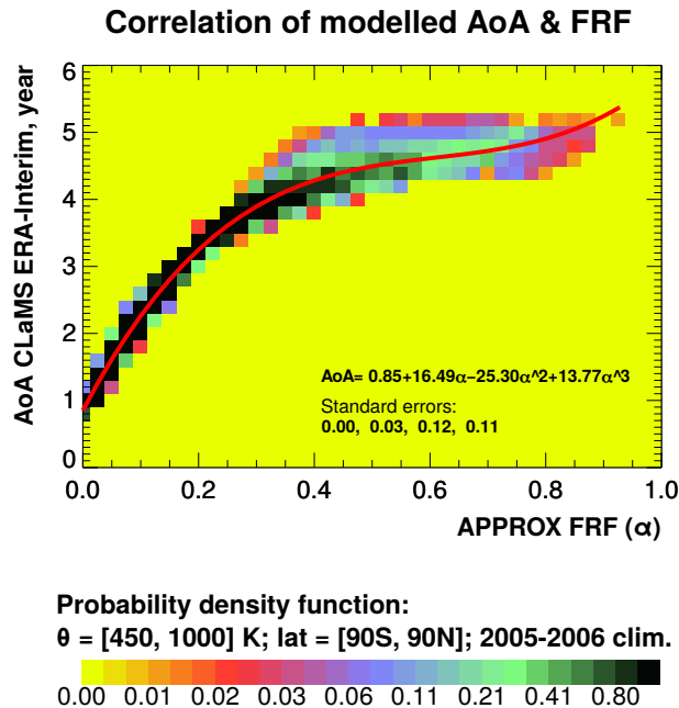
Figure A1. Relationship between CLaMS FRF and AoA for the methods of AoA trend estimation using stationary approximation. FRF is defined from the climatological 2005-2006 CLaMS simulated \text{CH}_4 , AoA is the climatological 2005-2006 from CLaMS simulations. The considered correlated region is between 450-1000 K and 90^\circ \text{ S} - 90^\circ \text{ N} . The colour bar represents the probability density function. The red line is a third-order polynomial fitting function.
