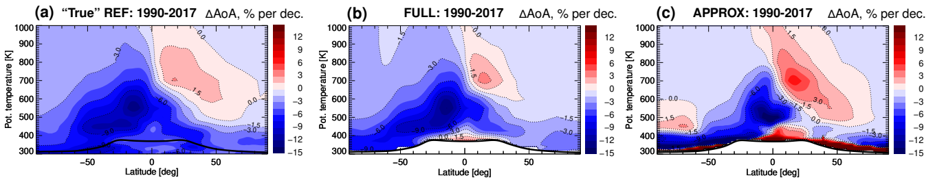
Figure 5. Decadal changes of AoA during 1990-2017: (a) "true" AoA changes from the CLaMS simulation driven by ERA-Interim reanalysis, (b) using CH 4 propagation by CLaMS age spectrum and monthly varying AoA-FRF correlation (FULL), (c) AoA changes estimated with the approximation method (APPROX). The changes are presented in percentage per decade relatively to the AoA 1990-2017 climatology in each used method of AoA calculation. The black line is the tropopause calculated from ERA-Interim.
