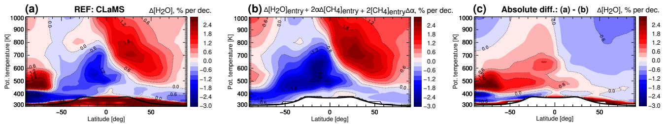
Figure 3. H 2 O trends during 1990-2017 period and their reconstruction, shown in percentage per decade with respect to the 1990-2017 climatology. Sub-figure (a) represents the reference (REF) “true” stratospheric H 2 O trend calculated from the CLaMS simulation driven by ERA-Interim reanalysis, (b) shows the reconstruction as sum of the different contributions from Fig. 2, (c) shows the absolute difference between (a) and (b). The black line is the tropopause calculated from ERA-Interim. Note, that due to the simple parameterisation of ice microphysics and the omission of a parameterisation of convective processes in CLaMS, the simulated H 2 O shown in (a) is meaningful only above the tropopause.
