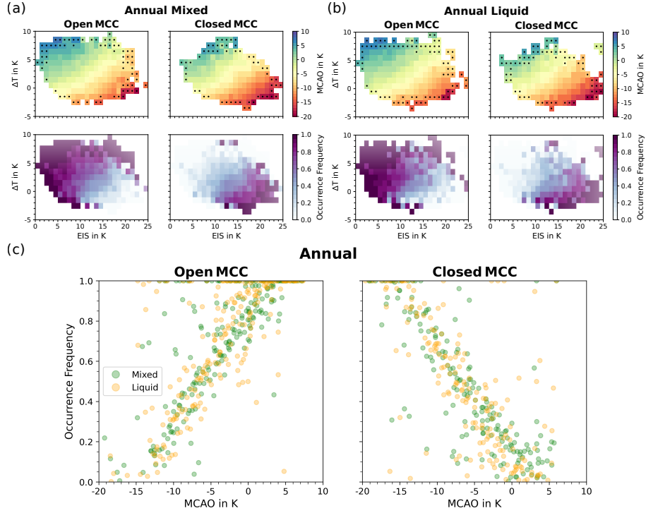
Figure S5. (a) Two-dimensional histograms of (top) the marine cold air outbreak (MCAO) and (bottom) occurrence frequency against \Delta T and EIS separately for (left) open MCC and (right) closed MCC MPCs. Dotted bins indicate bins with less than 100 data points. (b) Same as (a) but for SLCs. (c) \Delta T -EIS composites computed from the data in (a) for MPCs and (b) for SLCs separated in MPCs and SLCs for (left) open MCC and (right) closed MCC clouds binned by the MCAO index. This figure is produce in a similar way as from Fig. 8 and 9 by McCoy et al. (2017) but separately for MPCs and SLCs. [As MPCs and SLCs occur evenly across the MCAO index, the correlation between ice occurrence and vertical acceleration does not seem to be driven by surface fluxes.]
