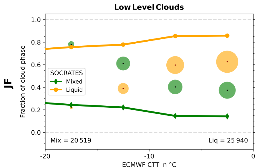
Figure S6. Supercooled liquid and mixed fraction binned by CTT from -20 °C to 0 °C with a bin width of 5 °C (2007 - 2010) for January and February in low level clouds. The months and region (42° S to 62° S and from 133° W to 163° W) are set to match the SOCRATES campaign. SOCRATES data is adapted from Fig. 4 by D'Alessandro et al. (2021).
