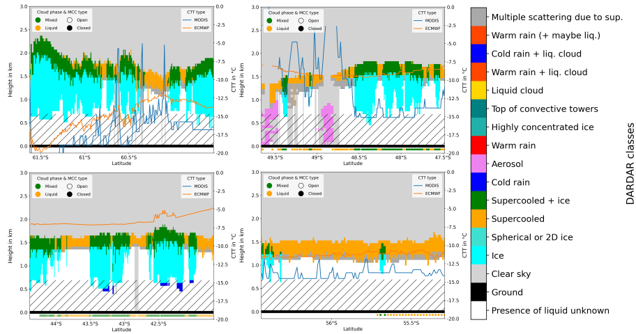
Figure S4. Four example tracks of the DARDAR categorization on 1 December 2007. The blue line indicates the CTT of MODIS and the orange of ECMWF. The hatched area displays levels below 720 m. The colored circles below the ground show the newly defined vertically integrated cloud phase and the MCC type for every other data point.
