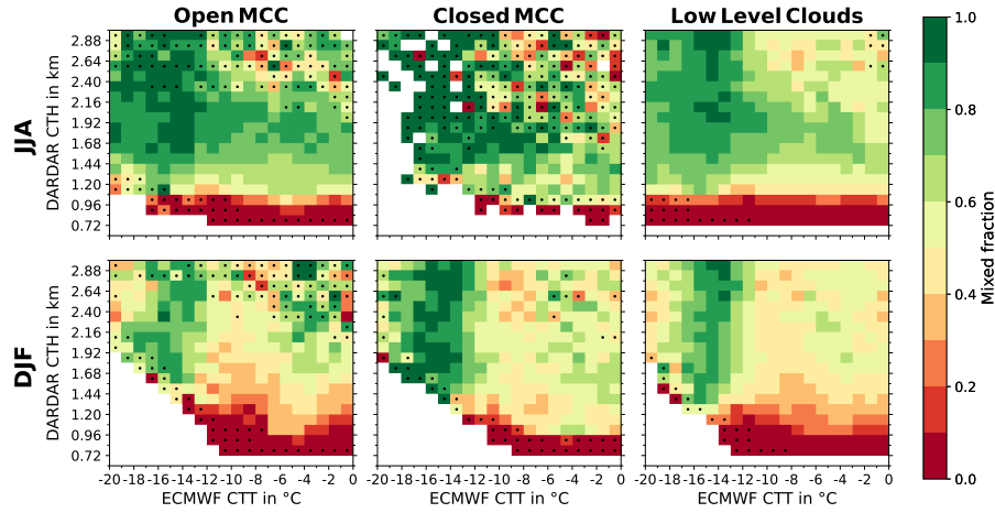
Figure S3. Two-dimensional histograms of mixed fraction against CTT and CTH for (left) open MCC, (middle) closed MCC, and (right) low level clouds in austral (top) winter and (bottom) summer. Dotted bins indicate bins with less than 100 data points.
