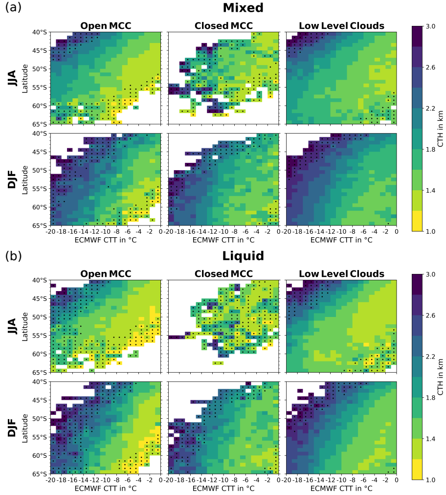
Figure S2. Two-dimensional histograms of CTH against CTT and latitude for (left) open MCC, (middle) closed MCC, and (right) low level clouds in (1. and 3. row) austral winter and (2. and 4. row) summer separately for (a) MPCs and (b) SLCs. Dotted bins indicate bins with less than 100 data points.
