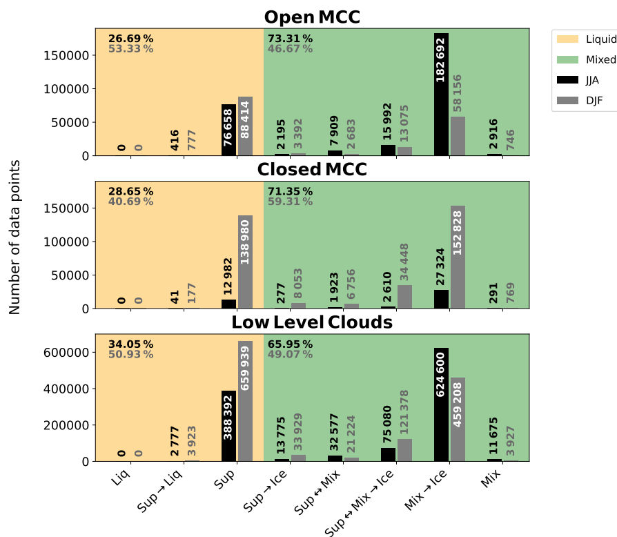
Figure S1. Histogram of data points of vertically resolved cloud phase types divided into two categories: liquid clouds (orange) and MPCs (green) for austral winter (black) and summer (grey) in the temperature range from -20^{\circ}\text{C} to 0^{\circ}\text{C} from 2007 to 2010. Overall percentage of liquid clouds and MPCs is indicated in each panel separately for JJA (black) and DJF (grey). "→" indicates layer on top of the next one. "↔" indicates interchangeable layers.
