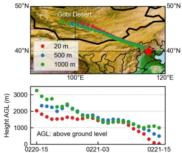
400 Figure A3. 24-hour back trajectory of the air parcel at the sampling site at three different heights (20 m, 500 m, and 1000 m above ground level).
