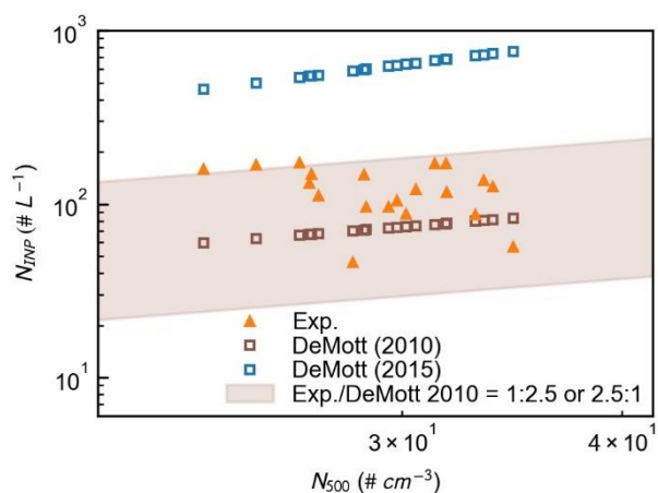
320 Figure 8: Inter-comparison of measured (solid orange triangles) and predicted (hollow blue and brown squares) N_{\text{INP}} during the dust event. The prediction is based on the parameterizations that link N_{\text{INP}} with the number concentration of particles larger than 500 nm ( N_{500} ) at a specific temperature (DeMott et al., 2010; DeMott et al., 2015).
