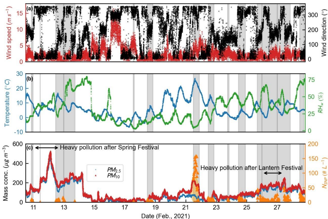
Figure 3: Times series of (a) wind speed and direction, (b) ambient temperature and relative humidity with respect to liquid water ( RH_w ), (c) PM_{2.5} and PM_{10} mass concentrations and immersion INP number concentration ( N_{INP} ). The grey shading in each panel indicates IN experiment time periods; the orange shading and arrows in the lower panel mark the dust event on Feb. 21 st , 2021 and the heavy pollution after celebrations, respectively.
