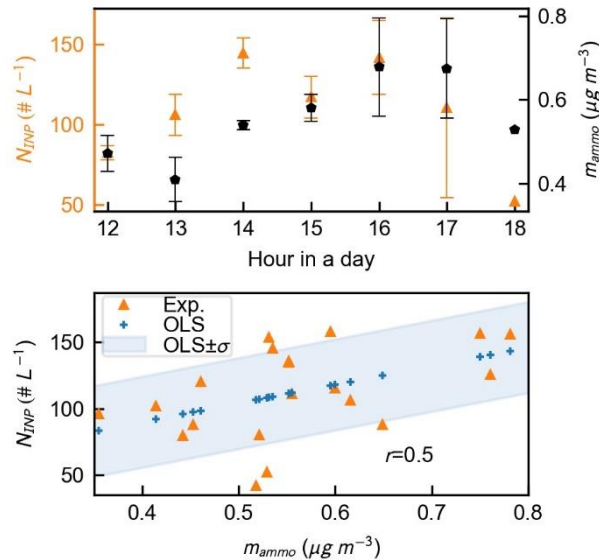
Figure 7: Diurnal profile of (upper panel) and correlation between (lower panel) N_{\text{INP}} and m_{\text{ammo}} during the dust event. The blue markers in the lower panel indicate the predicted N_{\text{INP}} using fitted linear regression parameters. The blue shading indicates \pm 1\sigma of measured N_{\text{INP}} from predicted N_{\text{INP}} .
