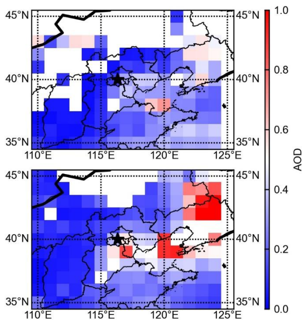
Figure A2. Aerosol optical depth (AOD) on Feb. 20 th (upper panel) and Feb. 21 st (lower panel) using MODIS Aqua Deep Blue Collection 6 aerosol data at 550 nm (Acker and Leptoukh, 2007). Sampling site is denoted with black star in each panel.
