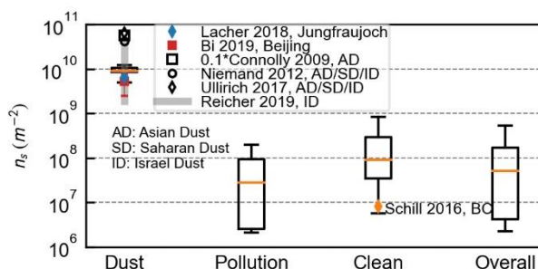
Figure 5: Ice-active surface site density ( n_s ) for different scenarios. The median (horizontal orange lines), 25 th and 75 th percentiles (lower and upper boxes), and 10 th and 90 th percentiles (lower and upper whiskers) are shown.
