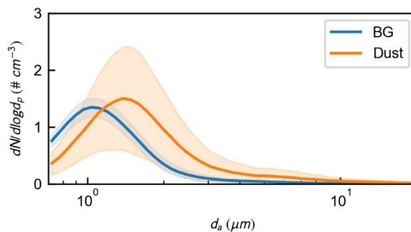
395 Figure A1. Aerodynamic diameter ( d_a ) size distribution of particles before (00:00-06:00, Feb. 21 st ; BG) and during the dust event (11:00-18:00, Feb. 21 st ; Dust).
