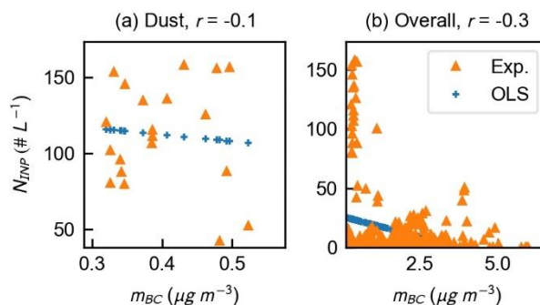
455 Figure C4: Correlations between m_{BC} and N_{INP} during the (a) dust event and (b) observation. r above each panel is Pearson's correlation coefficient. Blue markers indicate the predicted N_{INP} using fitted linear regression parameters.
