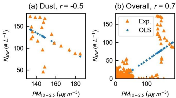
Figure C1: Correlations between PM_{10-2.5} and N_{INP} in the (a) dust event and (b) observation. r above each panel is Pearson's correlation coefficient. Blue markers indicate the predicted N_{INP} using fitted linear regression parameters.
