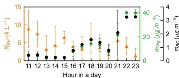
Figure 9: Mass concentration of organics ( m_{\text{org}} ) and BC ( m_{\text{BC}} ) on clean days.
