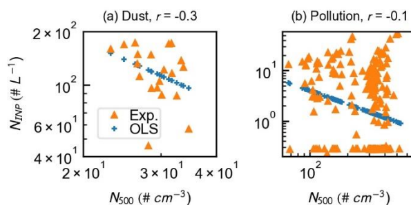
270 Figure 6: Correlations between N_{500} and N_{\text{INP}} for (a) dust event and (b) heavy pollution. r above each panel is the Pearson's correlation coefficient for the linear regression fitting of the experiment data using ordinary least square (OLS) method. Blue markers indicate predicted N_{\text{INP}} using fitted linear regression parameters.
