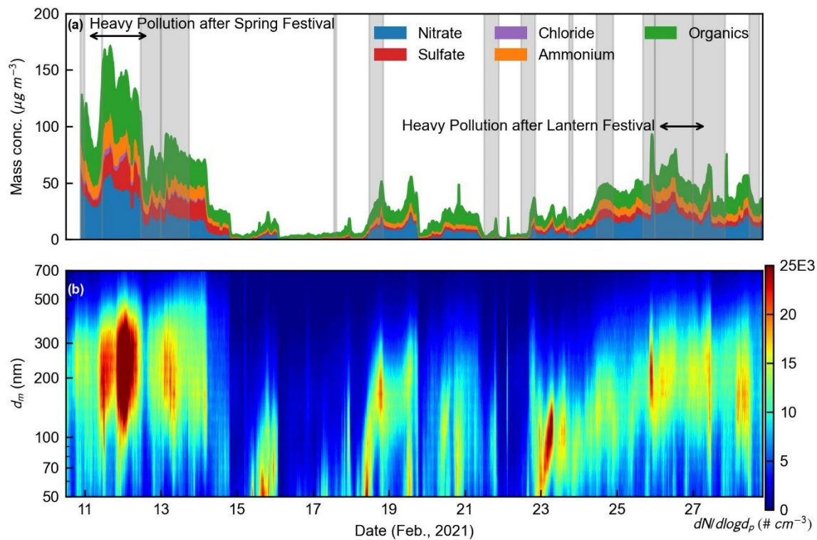
185 Figure 2: Time series of (a) non-refractory PM_1 mass concentration and (b) particle number size distribution. The grey shading and black arrows in the upper panel indicate IN experiment time periods and heavy pollution after celebrations, respectively.
