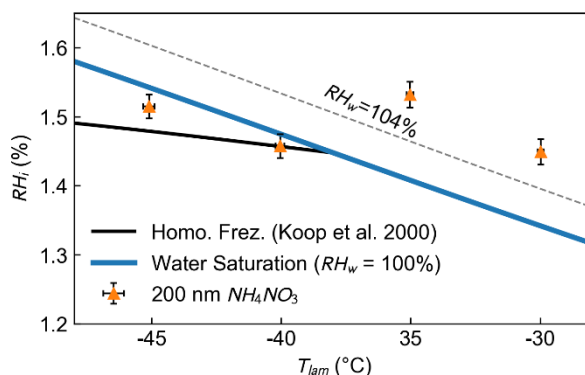
Figure B2. Phase diagram of the IN onset (below -38\text{ }^\circ\text{C} ) or water droplet detection in the >5\text{ }\mu\text{m} OPC channel (above -38\text{ }^\circ\text{C} ) for freezing or water droplet formation onto 200 nm dry diameter ammonium nitrate particles. The solid blue and black lines represent the water saturation line and the homogeneous freezing threshold of 200 nm aqueous droplets (Koop et al., 2000), respectively. The horizontal and vertical error bars represent the variation of temperature and RH_i along HINC lamina centerline.
