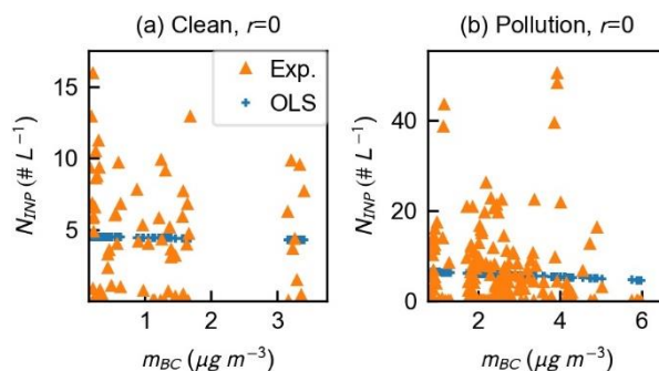
Figure 10: Correlations between m_{BC} and N_{INP} during (a) clean and (b) heavy pollution periods. R^2 above each panel is Pearson's correlation coefficient. Blue markers indicate the predicted N_{INP} using fitted linear regression parameters.
