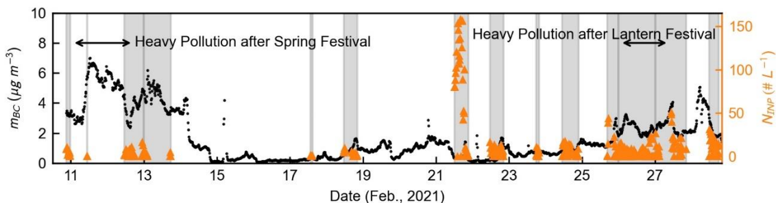
Figure 4: Time series of black carbon (BC) particle mass concentration ( m_{BC} ) and N_{INP} . The grey shading and black arrows indicate IN experiment time periods and heavy pollution after celebrations, respectively.
