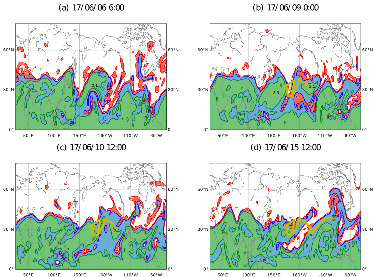
Figure 3. Example of the indirect transport pathway from the ASMA into the lower-stratosphere by two eastward shed cutoffs from the ASMA at 380K. Colors are as in Fig. 2. Yellow lines show tracks of the 4.0 PVU cutoffs. The largest cutoff (3.26% of NH) remains only a very short time over the West Pacific. The smaller cutoff (2.12% of NH) has a very long lifetime of about one week and travels to North America.
