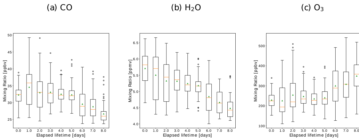
Figure 11. Chemical evolution of the chemical species (a) CO, (b) H 2 O and (c) O 3 along the exemplary PV cutoff shown in Fig. 10. Box and whisker plots are as in Fig. 9.
