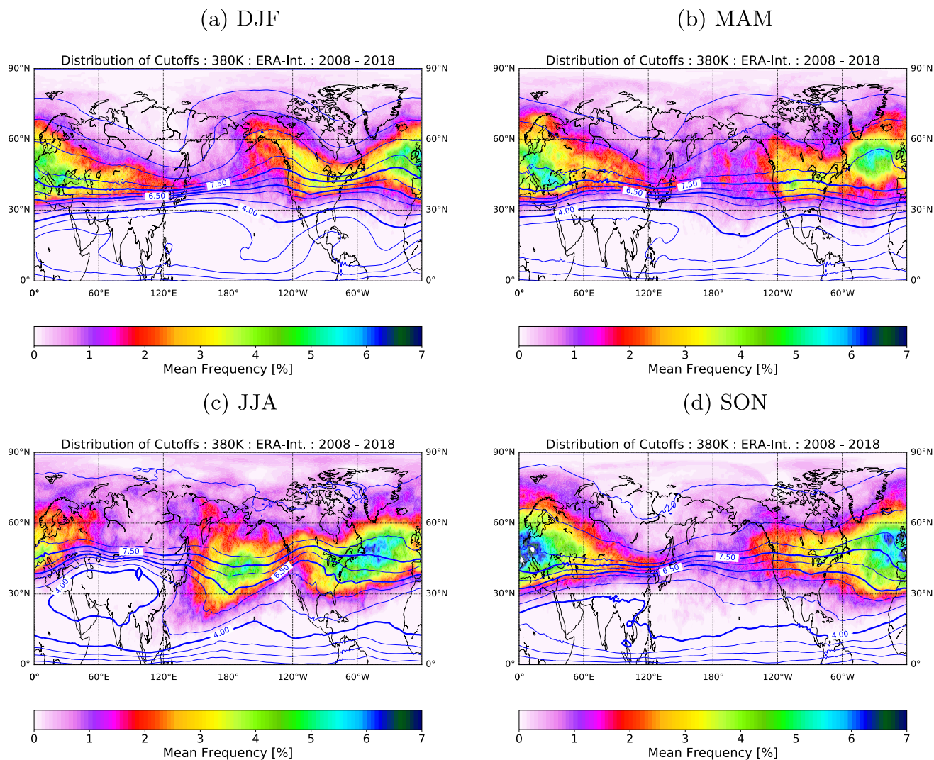
Figure 4. Global climatological frequency distribution of 6.5 PVU cutoffs in the four seasons. A frequency of 1% percent mean frequency means that during a season in 1% of the time-steps, a cutoffs covers the point.
