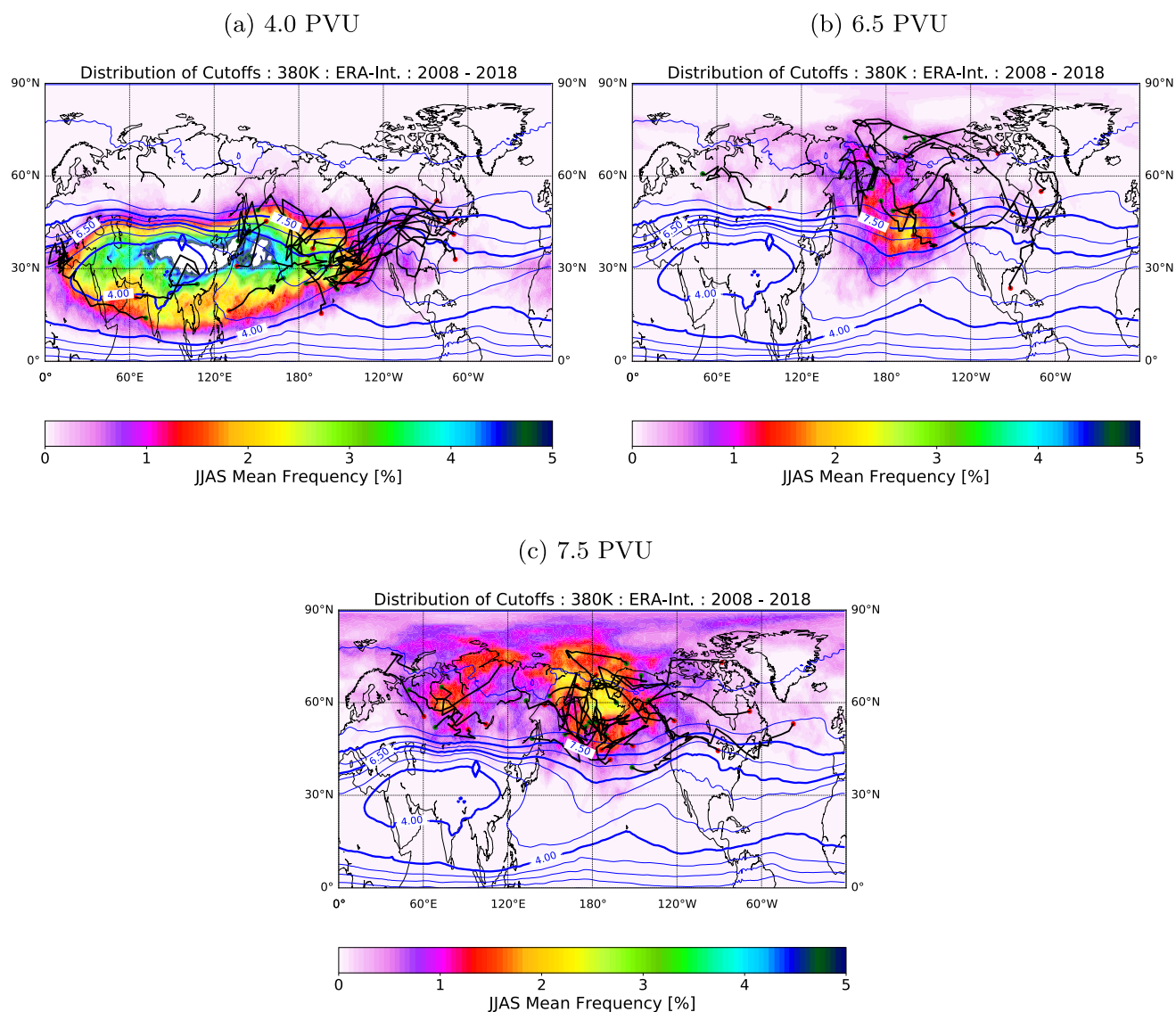
Figure 5. Climatological frequency of ASMA-related cutoffs during JJAS, for (a) 4.0 PVU cutoffs, (b) 6.5 PVU cutoffs and (c) 7.5 PVU cutoffs. The blue lines indicate particular PV contours. A subset of the identified tracks with a lifetime of at least 4 days is plotted with black lines, where green dots symbolize the starting points and red dots the end points of the tracks. Here, 1% means that a point is covered with a cutoff in 1% of the time steps in JJAS.
