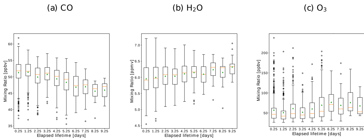
Figure 9. Chemical evolution of the chemical species (a) CO, (b) H 2 O and (c) O 3 within the exemplary PV cutoff of Fig. 3. The box and whisker plots show the upper and lower quantile, the median (orange line) and the average (green pyramid) of the mixing ratios for each time step during the lifetime of the PV cutoff cascade. The black dots show outliers.
