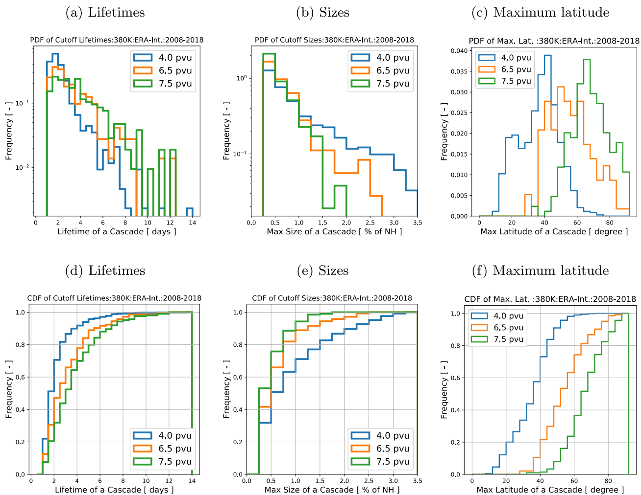
Figure 6. PDFs (top row) and CDFs (bottom row) for the lifetime, size and maximum latitude of ASMA-related cutoffs at 380K between 2008 and 2018. The frequencies are determined from the number of cutoffs.
