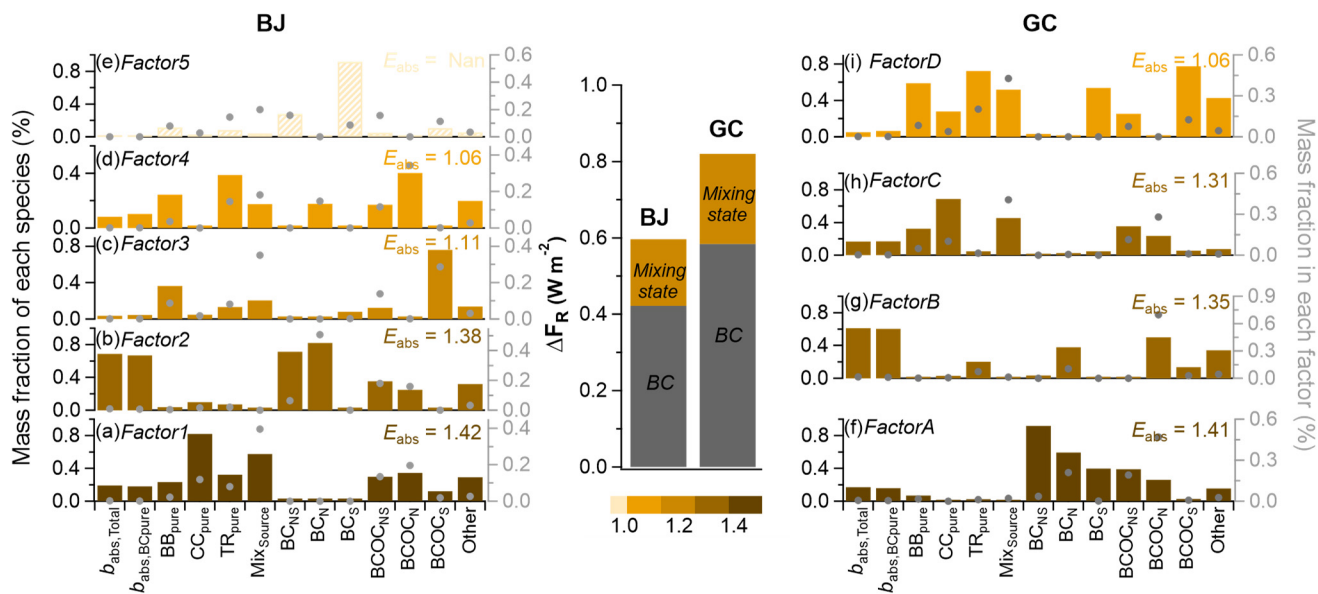
530 Figure 5. Factor profiles and their contributions to each factor identified by the positive matrix factorization model in Beijing and Gucheng. b_{\text{abs, total}} and b_{\text{abs, BCpure}} represent light absorption ( \text{Mm}^{-1} ) of coated BC particles and pure BC, respectively. BC types e.g., \text{BB}_{\text{pure}} in units of count.
