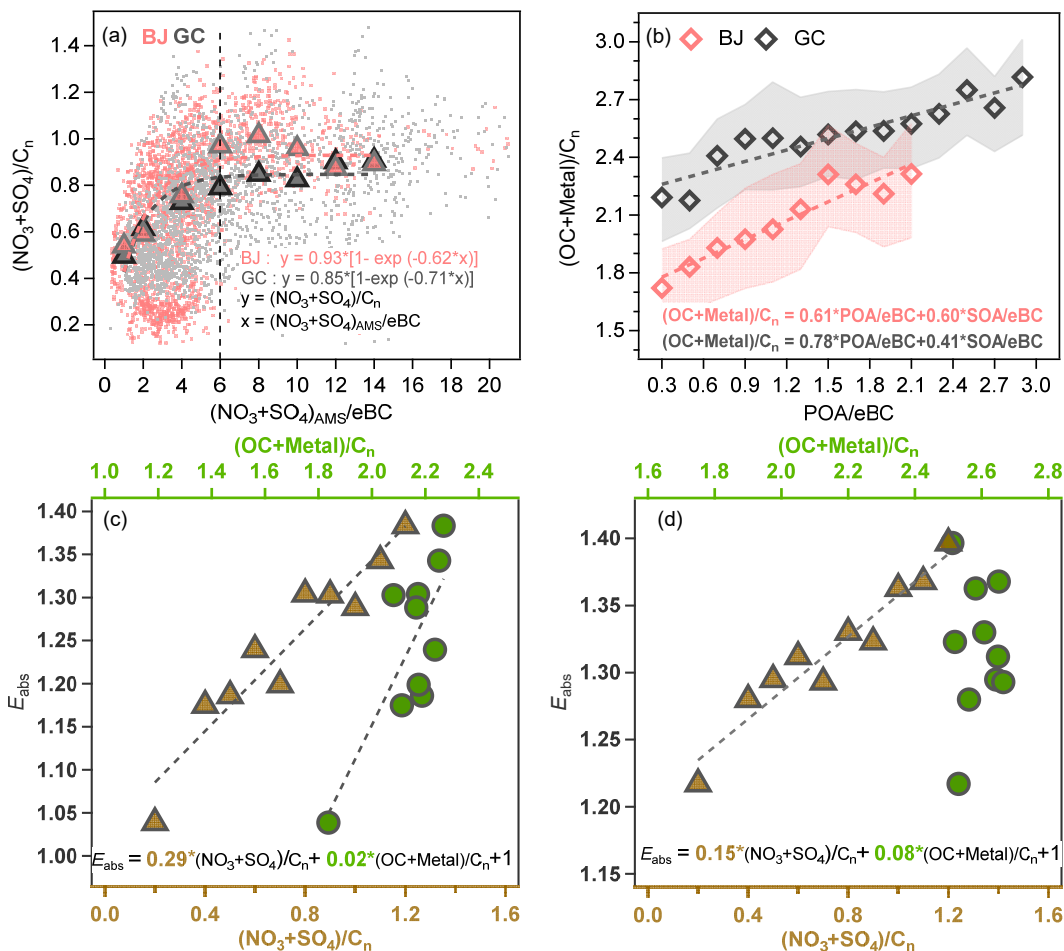
Figure 4. Relationships between peak area ratios and mass concentration ratios (a) (\text{NO}_3 + \text{SO}_4)/C_n vs. (\text{NO}_3 + \text{SO}_4)_{\text{AMS}}/e\text{BC} and (b) (\text{OC} + \text{Metal})/C_n vs. \text{POA}/e\text{BC} . Relationships between E_{\text{abs}} and peak area ratios of coating materials (\text{NO}_3 + \text{SO}_4)/C_n and (\text{OC} + \text{Metal})/C_n in (c) Beijing and (d) Gucheng. The triangles in (a) are the averages of different bins that are grouped according to (\text{NO}_3 + \text{SO}_4)_{\text{AMS}}/e\text{BC} . The rhombuses in (b) are the averages of different bins that are grouped according to \text{POA}/e\text{BC} . The shades areas in (b) indicate 25th and 75th percentiles of the (\text{OC} + \text{Metal})/C_n ratios. The triangles and circles in (c) and (d) are the averages of different bins that are grouped according to (\text{NO}_3 + \text{SO}_4)/C_n .
