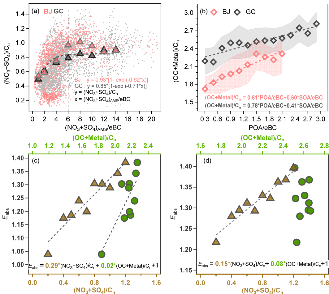
Figure 4. Relationships between peak area ratios and mass concentration ratios (a) (NO_3 + SO_4)/C_n vs. (NO_3 + SO_4)_{AMS}/eBC and (b) (OC + Metal)/C_n vs. POA/eBC . Relationships between E_{abs} and peak area ratios of coating materials (NO_3 + SO_4)/C_n and (OC + Metal)/C_n in (c) Beijing and (d) Gucheng. The triangles in (a) are the averages of different bins that are grouped according to (NO_3 + SO_4)_{AMS}/eBC . The rhombuses in (b) are the averages of different bins that are grouped according to POA/eBC . The shades areas in (b) indicate 25th and 75th percentiles of the (OC + Metal)/C_n ratios. The triangles and circles in (c) and (d) are the averages of different bins that are grouped according to (NO_3 + SO_4)/C_n .
