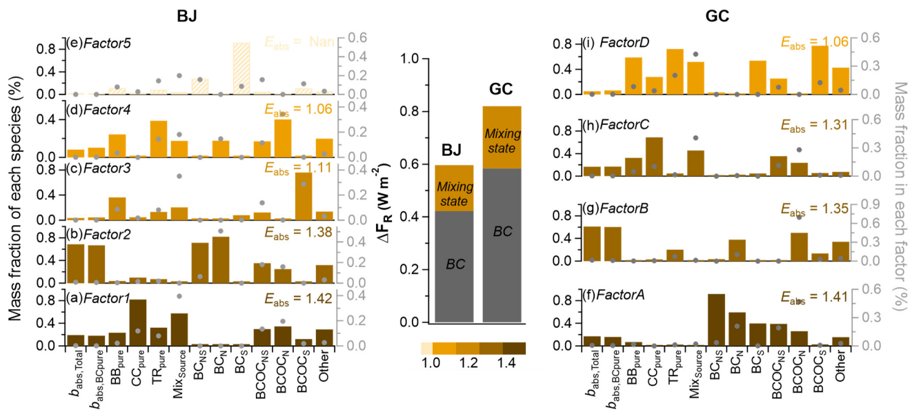
Figure 5. Factor profiles and their contributions to each factor identified by the positive matrix factorization model in Beijing and Gucheng. b_{\text{abs, total}} and b_{\text{abs, BCpure}} represent light absorption ( \text{Mm}^{-1} ) of coated BC particles and pure BC, respectively. BC types e.g., \text{BB}_{\text{pure}} in units of count.
