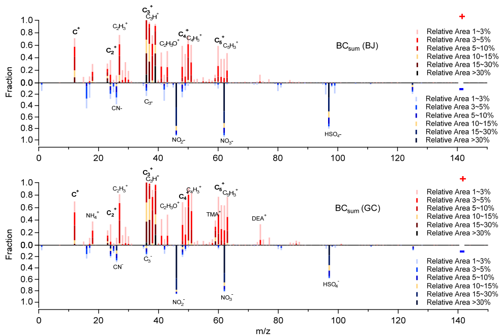
Figure 1. The digital Digital positive and negative mass spectra of BC-containing particles in Beijing and Gucheng. The ion height indicates its number fraction in the BC-containing dataset (i.e., the number ratio of BC-containing particles with the corresponding ion detected in the mass spectra to the total BC-containing particles). The color bars represent each relative peak area corresponding to a specific fraction in the individual particles.
