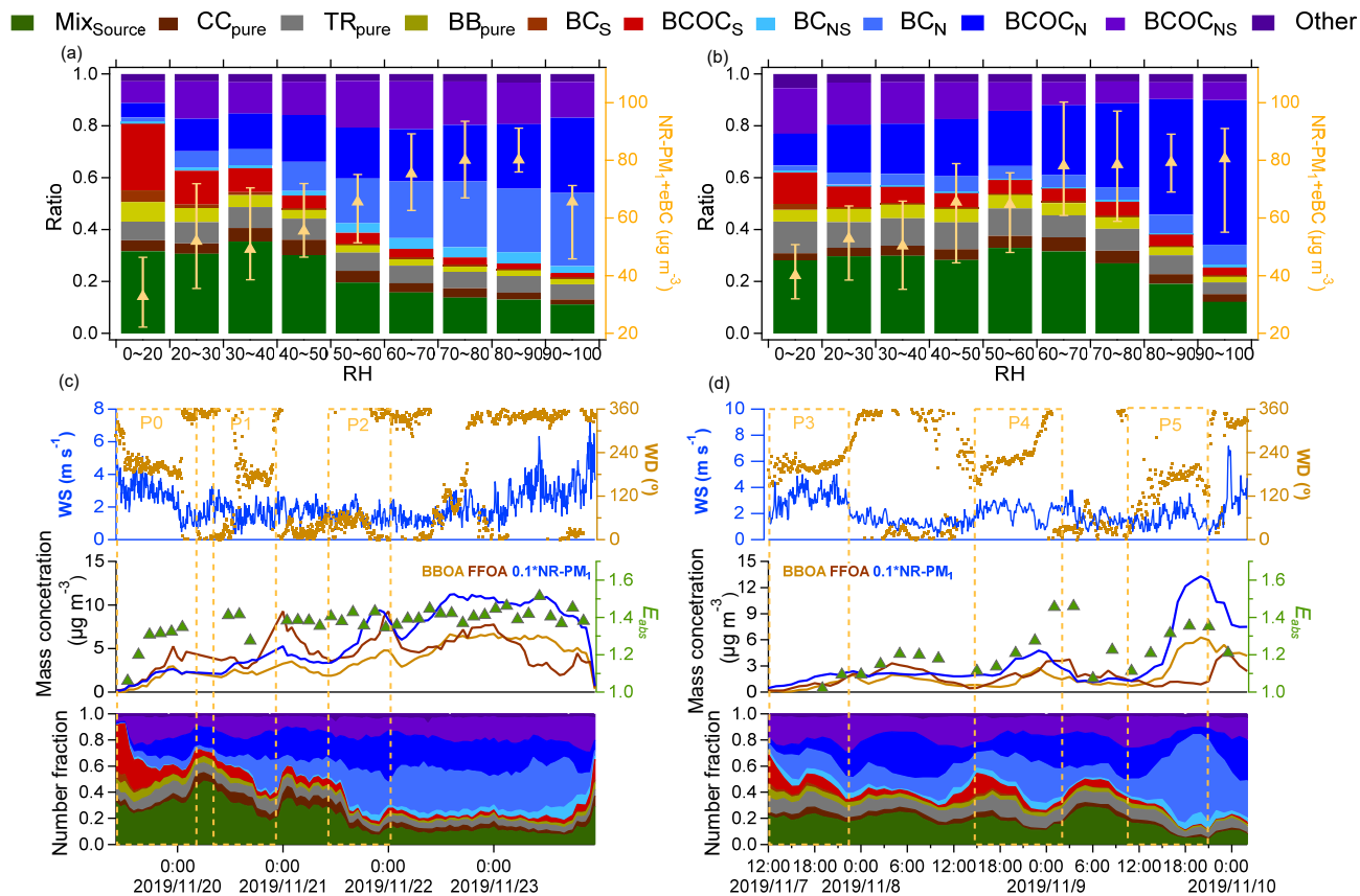
520 Figure 3. Variations of number fractions of BC-containing particle types with RH in (a) Beijing and (b) Gucheng. The bottom and top error bars represent 25th and 75th percentiles. Temporal variations of wind speed (WS), wind direction (WD), E_{abs} , number fractions of BC-containing particle types and mass concentration of species during polluted (c) Case1 and (d) Case2 in Beijing.
