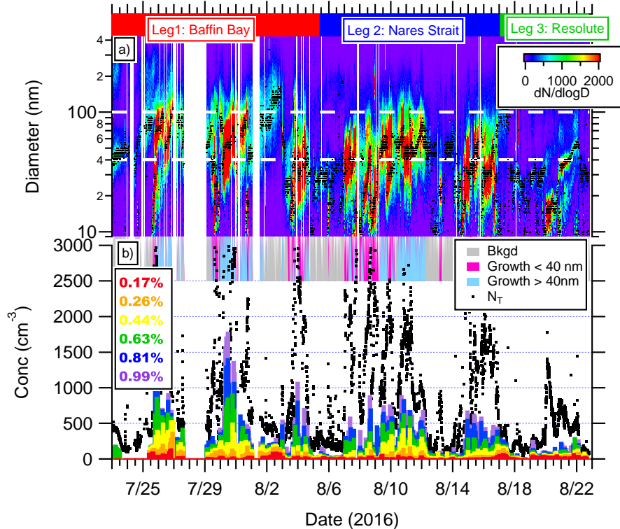
Figure 2. Time series of a) aerosol number size distribution and D_{max} (black points) and b) N_T (black points) and CCN concentrations. Dashed white horizontal lines show particle diameters of 40 and 100 nm. Times used in calculations of Background, Growth > 40 nm and Growth < 40 nm are shown in grey, light blue, and magenta, respectively.
