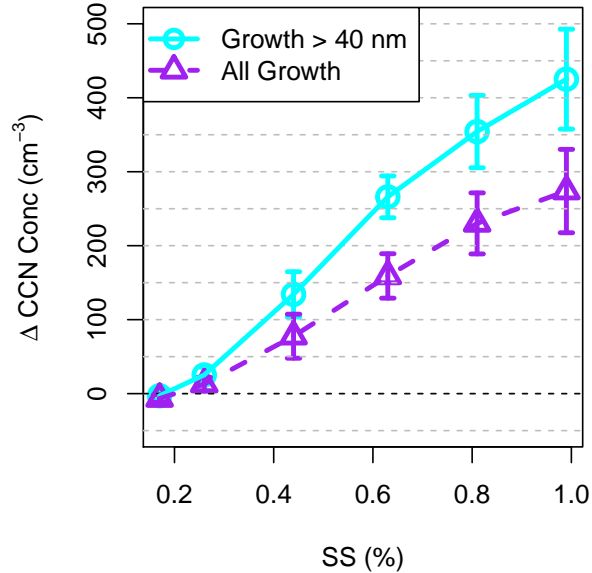
Figure 5. The increase in CCN concentration during Growth > 40 nm (cyan) and All Growth (purple) times compared to Background times at different SS. The error bars show the 95% confidence interval.
