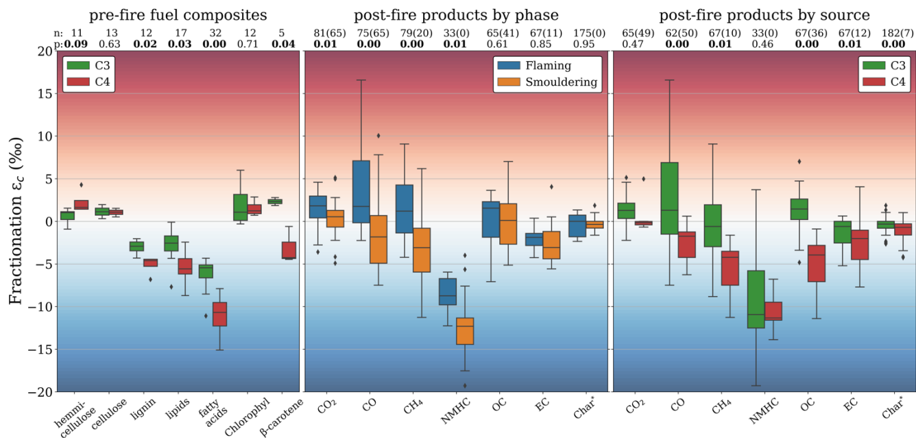
Figure 7: Left: \delta^{13}\text{C} fractionation of various sub-compounds of the fuel compared to the bulk plant (i.e. the combined sub-compounds) for C3 (green) and C4 (red) vegetation. Middle: \delta^{13}\text{C} fractionation in pyrolysis products for flaming (blue) and smouldering (orange) combustion phases. Right: \delta^{13}\text{C} fractionation in pyrolysis products for C3 (green) and C4 (red) vegetation. The first row of numbers over the boxplots (n) represent the number of individual \delta^{13}\text{C} measurements taken from literature and from this study combined, with the number from this study in parentheses. The second row (p) represents P-value calculated using a two-tailed t test with unequal variance.
