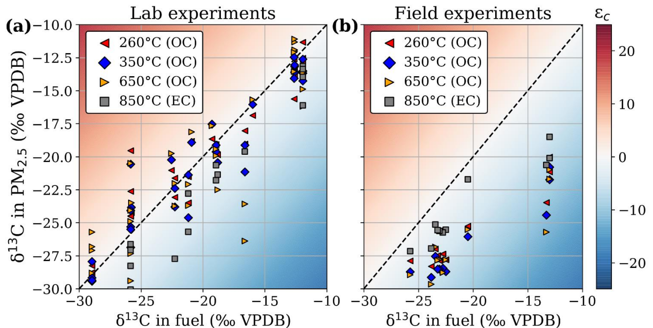
Figure 5: The \delta^{13}\text{C} measured in the different volatility fractions of the captured PM 2.5 versus \delta^{13}\text{C} in the fuel for lab experiments (a) and samples from landscape fires in Mozambique (b). The temperature classes refer to the evaporation temperature steps in the oven of the organic carbon (OC) / elemental carbon (EC) analyser.
