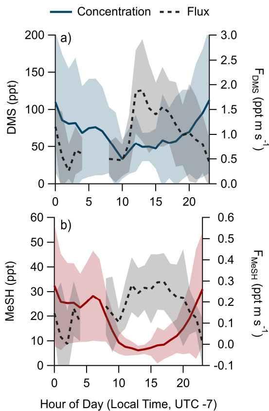
Figure 4. Hourly averaged diel profiles of observed mixing ratios and eddy covariance flux of (a) DMS and (b) MeSH. Shading represents the standard deviation of the binned hourly means. Winds were primarily from the land for hours 0 to 10, limiting air-sea flux measurement during those times.
