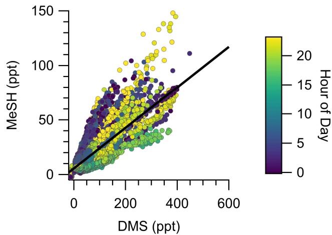
Figure 3. Correlation of DMS and MeSH mixing ratios at a 2 minute averaging time colored by hour of day of the observation. Hour of day is in local time (UTC -7). The linear least-squares best fit is plotted as the solid black line. The slope of the best fit line is 0.19 and R^2 = 0.61 .
