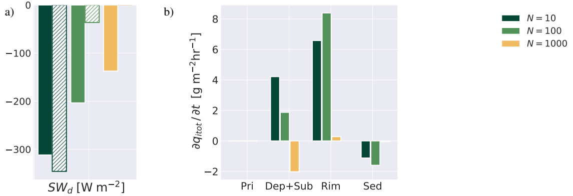
Figure 15. Bar plots of the effects of cloud processes. a) the comparison of the short wave downward flux estimated from Twomey formula (shown as bars with the pattern ) and the short wave downward flux from the from the simulation output (shown as full coloured bars); b) Vertically integrated tendencies in (total) ice water mass budget within the cloud layer: primary ice nucleation and freezing of cloud droplets (Pri, significantly smaller than other tendencies), the combined effect of deposition and sublimation (Dep+Sub), riming of cloud droplets (Rim), and sedimentation (Sed). The time-averaging covers the last 48 hours of the simulations.
