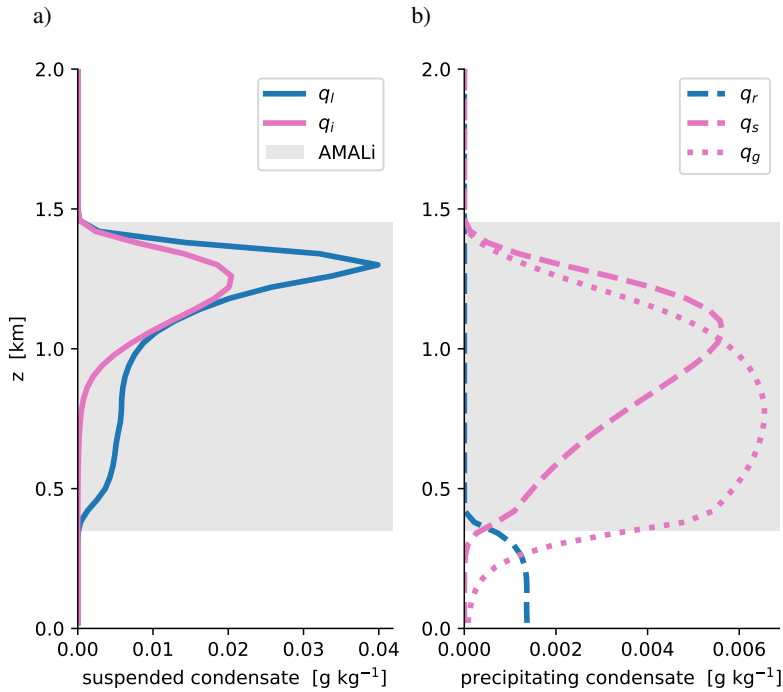
Figure 8. The specific masses of all five hydrometeor species in the control simulation at t = 24 hr. a) Suspended species, including liquid water q_l and ice water q_i . b) Precipitating species, including rain q_r , snow q_s and graupel q_g . Liquid species are shown in blue, frozen species in pink. The vertical range of AMALi cloud top heights sampled within the target domain as shown in Fig. 2 is shaded grey.
