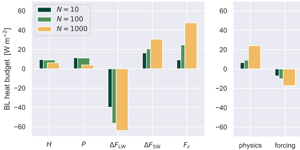
Figure 17. Analysis of the bulk heat budget of the boundary layer below the base of the capping inversion. a) Bar plot of all physics terms in the sensible heat budget, plotted as energy fluxes. b) The net contribution by all physics terms as shown in a) and the large-scale forcing h\dot{\theta}_{\text{LS}} .
