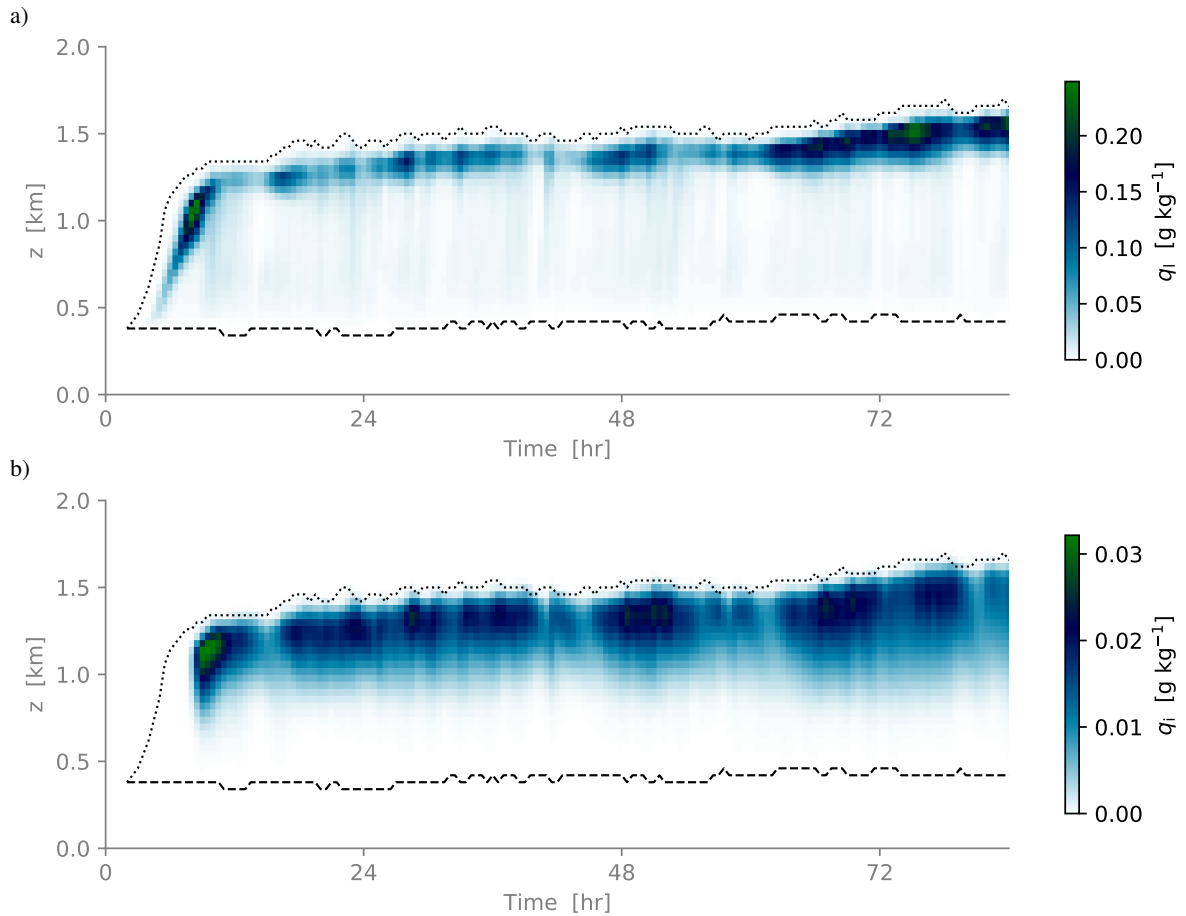
Figure 5. Time-height contour plots of domain-averaged variables during the control experiment. Mass concentration of a) cloud liquid water q_l , b) cloud ice water q_i . The averaging time is 30 min. The dashed and dotted lines reflect the lowest base and highest top of liquid clouds in the domain, respectively.
