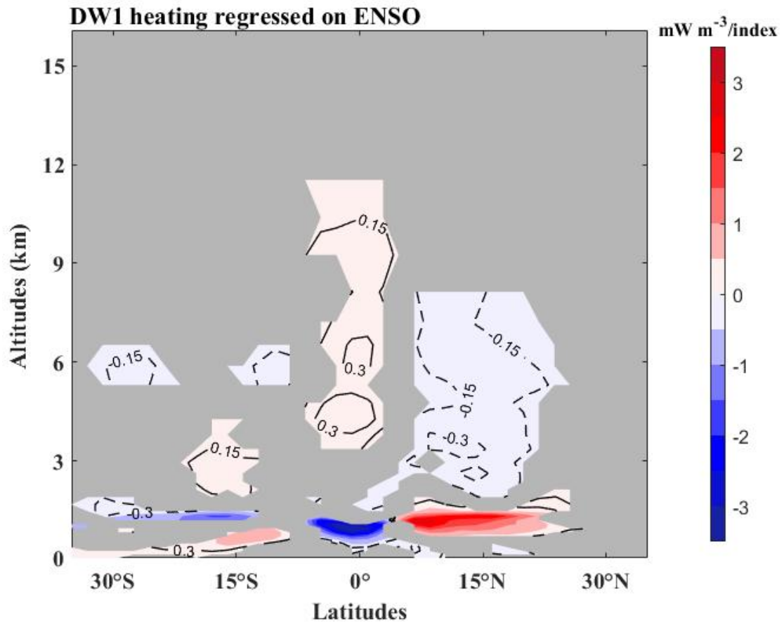
Figure 5. The linear regression coefficient of normalized Niño3.4 in SD-WACCM heating amplitude ( \text{mW/m}^3 per index) during 1979-2013 winters (DJF). Solid lines and red shadings denote the positive responses, while dashed lines and blue shadings denote the negative responses; the grey regions indicate where the response is insignificant at the 95% level according to the F test.
