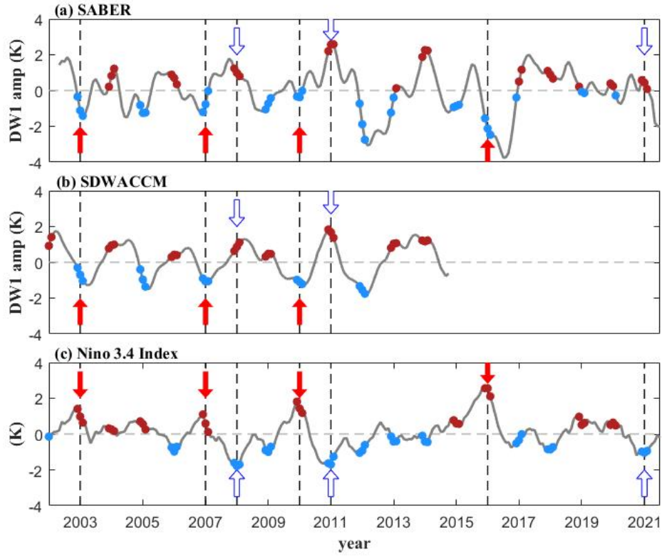
Figure 2. (a) The residual DW1 temperature amplitude of SABER observations averaged over 10°S-10°N at 100 km from 2002 to 2021. (b) Same as in (a) but for SD-WACCM. (c) Niño3.4 index. Dashed lines represent ENSO events. The red solid and hollow blue arrows denote the El Niño and La Niña events.
