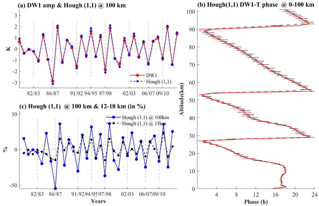
Figure 4. (a) The red line indicates the anomalous DW1 temperature amplitude of SD-WACCM simulations averaged over 10°S-10°N at 100 km during the 1979-2013 winter (DJF). The blue line indicates the Hough (1,1) mode of the DW1 temperature amplitude residual at 100 km during the 1979-2013 winter (DJF). (b) The thin black line indicates the Hough (1,1) DW1-T phase of SD-WACCM simulations at 0-100 km during the 1979-2013 winter (DJF). The thick black horizontal line indicates the standard deviation of the DW1-T phase. The red line is the same but for El Niño winter. (c) The blue line is the same as in (a), and the black line is the same but for 15 km.
