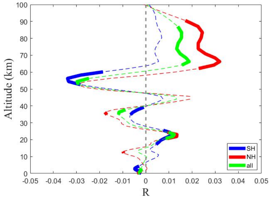
Figure 6. The linear regression coefficient of normalized Niño3.4 in \delta R (the anomaly of the ratio of the absolute and to planetary vorticity). The thin, dashed red, blue, and green lines denote the averages of the Northern Hemisphere (from 15°N to 30°N), Southern Hemisphere (from 15°S to 30°S), and the whole (15-30°N and 15-30°S), respectively. The thick, solid lines denote confidence levels below higher than 95% for the F test.
