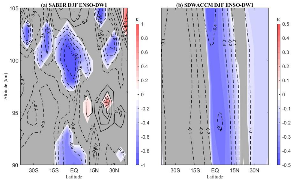
Figure 3. The linear regression coefficient of normalized Niño3.4 in SABER (a) and SD-WACCM (b) winter DW1-T. The contour interval is 0.2 K for SABER and 0.1 K for SD-WACCM. Red represents a Solid lines and red shadings denote the positive response, responses, while dashed lines and blue represents a shadings denote the negative response responses; the grey regions denote confidence levels below indicate where the response is insignificant at the 95% for level according to the F test.
