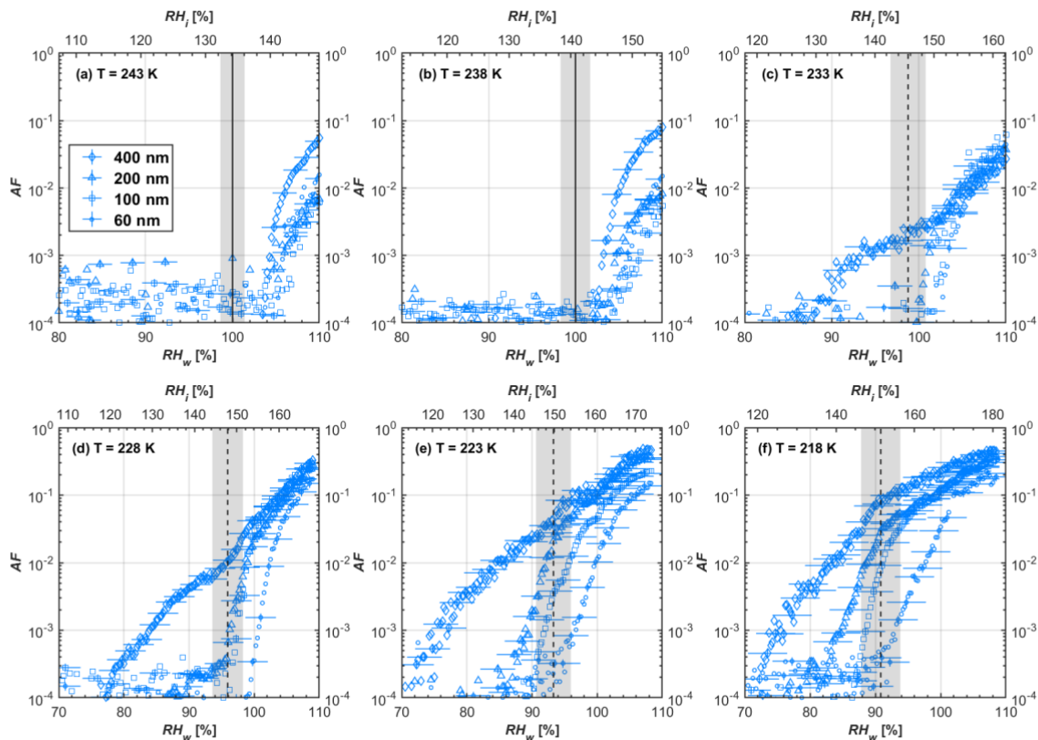
960 Figure C5. Averaged AF curves as a function of RH_w and RH_i from the 1\ \mu\text{m} OPC channel for size selected fresh FW200 soot particles at different T . Black solid lines represent water saturation conditions according to Murphy and Koop (2005). Black dashed lines denotes the expected RH values for solution droplet homogeneous freezing at each T (Koop et al., 2000). The grey shading shows the possible variation range in RH that aerosol in HINC can encounter for the calculated homogeneous freezing RH values at each T .
