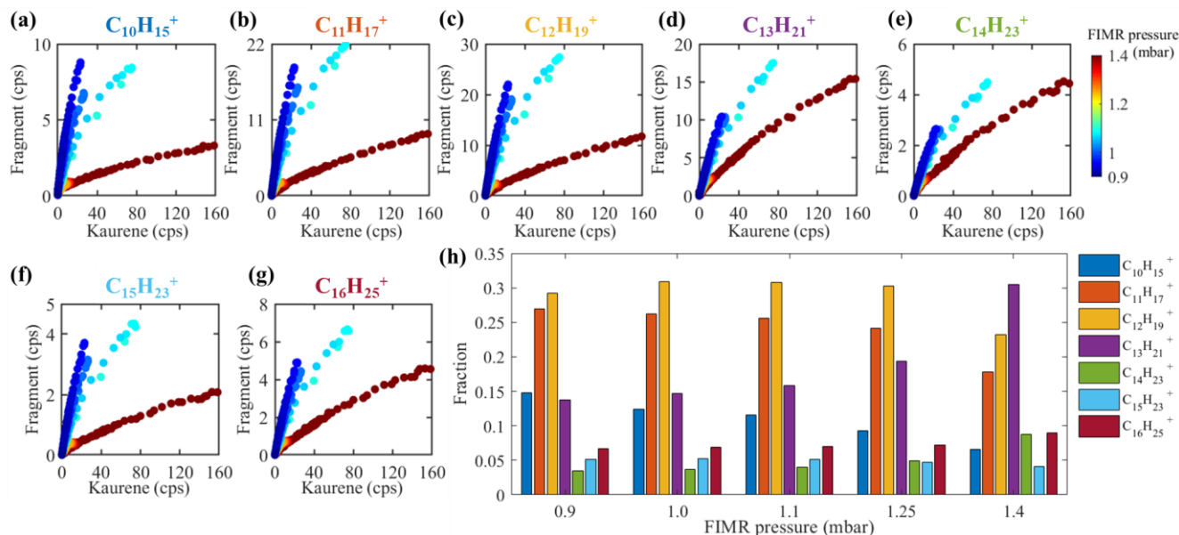
760 Figure 7. Fragments in Vocus. Panels (a)-(g) show the relationship between the signals of kaurene and its fragments in Vocus. Kaurene and its fragments are shown with raw signal intensities without corrections, colored with FIMR pressures ranging from 0.9 to 1.4 mbar. Panel (h) shows the fraction of the fragments as a function of FIMR pressures in Vocus. (fraction = signal of fragment / total signal of all fragments).
