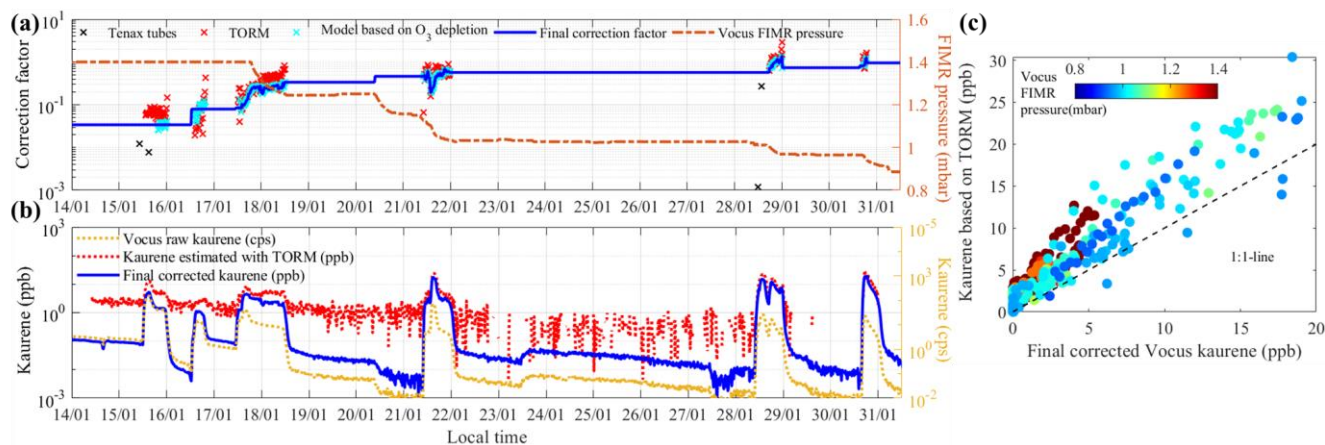
Figure 1. Correction factors and time series of kaurene. Panel (a) shows the correction factors (left axis) needed to scale the Vocus count rates to mixing ratios at varying FIMR pressures (right axis) using different methods. The black crosses represent the needed correction factors based on Tenax tube samples, the red crosses represent correction factors derived from the TORM system, and the blue crosses represent correction factors according to the O 3 depletion model (see Sect. 2.3 for details). The blue line shows the final correction factors we used in this study. Panel (b) displays the time series of the measured raw kaurene signal intensities (yellow), the kaurene concentration estimated by the O 3 reactivity system TORM (red), and the final kaurene concentration after corrections (blue). Panel (c) shows the relationship between the kaurene concentrations based on the TORM system and the final corrected Vocus kaurene concentrations.
