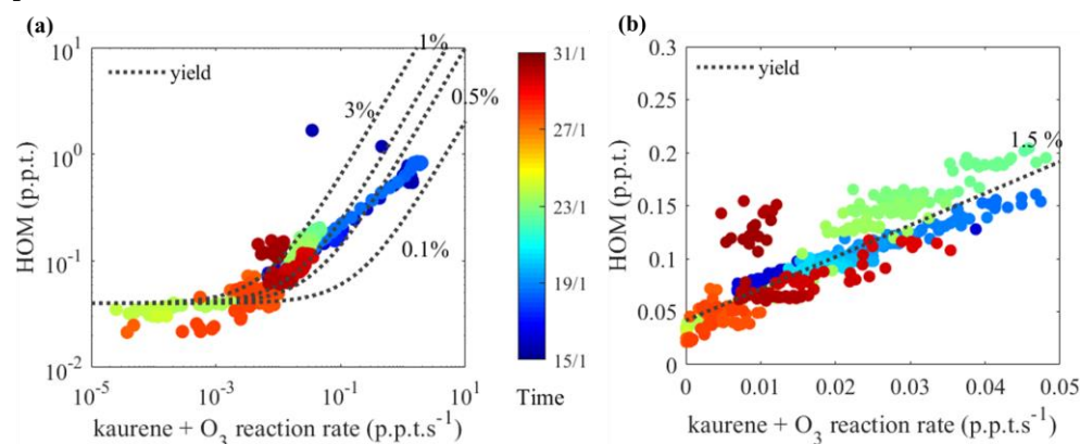
745 Figure 5. HOM yield estimation. HOM concentrations were plotted against the kaurene ozonolysis rate in panels (a) and (b). Markers are colored by time, representing the changes of calibration factors applied to kaurene signals. Lines are added to the plots to represent constant HOM molar yields from kaurene ozonolysis, accounting for an instrumental HOM background in the CI-APi- TOF of 0.04 ppt. (a) All data points (plotted in logarithmic scale) from the periods without seed particles in the chamber. A zoomed- in view of panel (a) with reaction rates ranging from 0 to 0.05 ppt s^{-1} is shown in panel (b) (plotted in linear scale).
