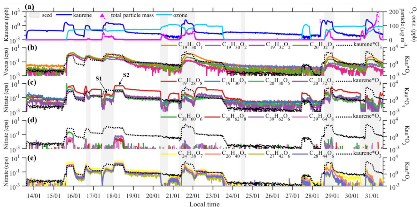
Figure 3. Overview of the measurements from January 13th to 31st, 2020. Panel (a) shows O_3 and corrected kaurene concentrations and the total particle mass calculated from SMPS and AMS measurements. Some of the most abundant oxidation products measured with Vocus are shown in panel (b). HOM monomers and dimers of kaurene ozonolysis detected by nitrate CI-API-TOF are shown in panels (c)–(e). The light gray shade indicates periods when there were seed particles in the chamber. The black dashed lines are included in each panel to depict the kaurene ozonolysis rate ( Kau \cdot O_3 in the right y-axis representing kaurene concentration times O_3 concentration, in units ppb^2 ). The ‘S1’ and ‘S2’ mark two steady-state periods used to determine the condensation behavior of oxidation products (Sect. 3.3).
