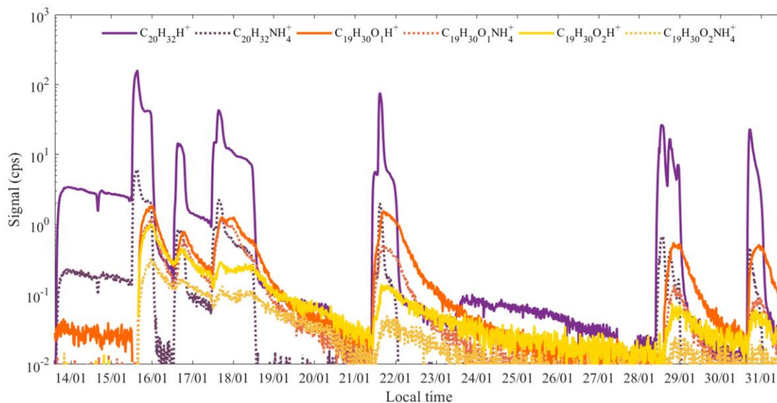
765 Figure 8. Comparison of the measured time series of kaurene and two oxidation products detected as protonated or adducts with \text{NH}_4^+ . Both the protonated and \text{NH}_4^+ cluster signals are raw data without FIMR pressure corrections.
