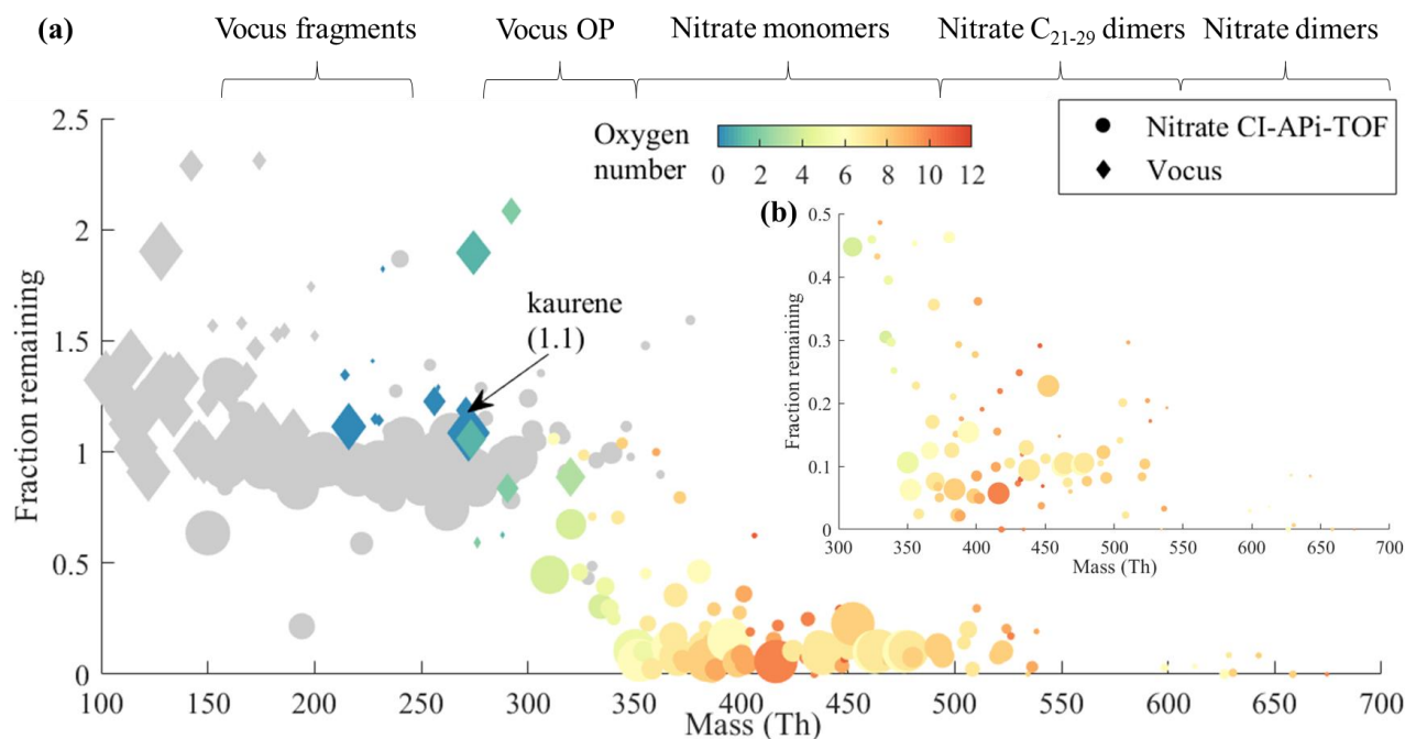
750 Figure 6. Seed injection behaviour. The “fraction remaining” corresponds to the ratio of the signal with seed particles to the signal without seed. We emphasize that the molar mass indicated on the x-axis is without the reagent ions, unlike many previous studies (Peräkylä et al., 2020; Rätty et al., 2021). Species with less than 15 carbon numbers in the composition are colored with gray, while the color scale indicates the oxygen content for species with 15 or more carbon atoms. The area of circles (nitrate CI-APi-TOF) and
