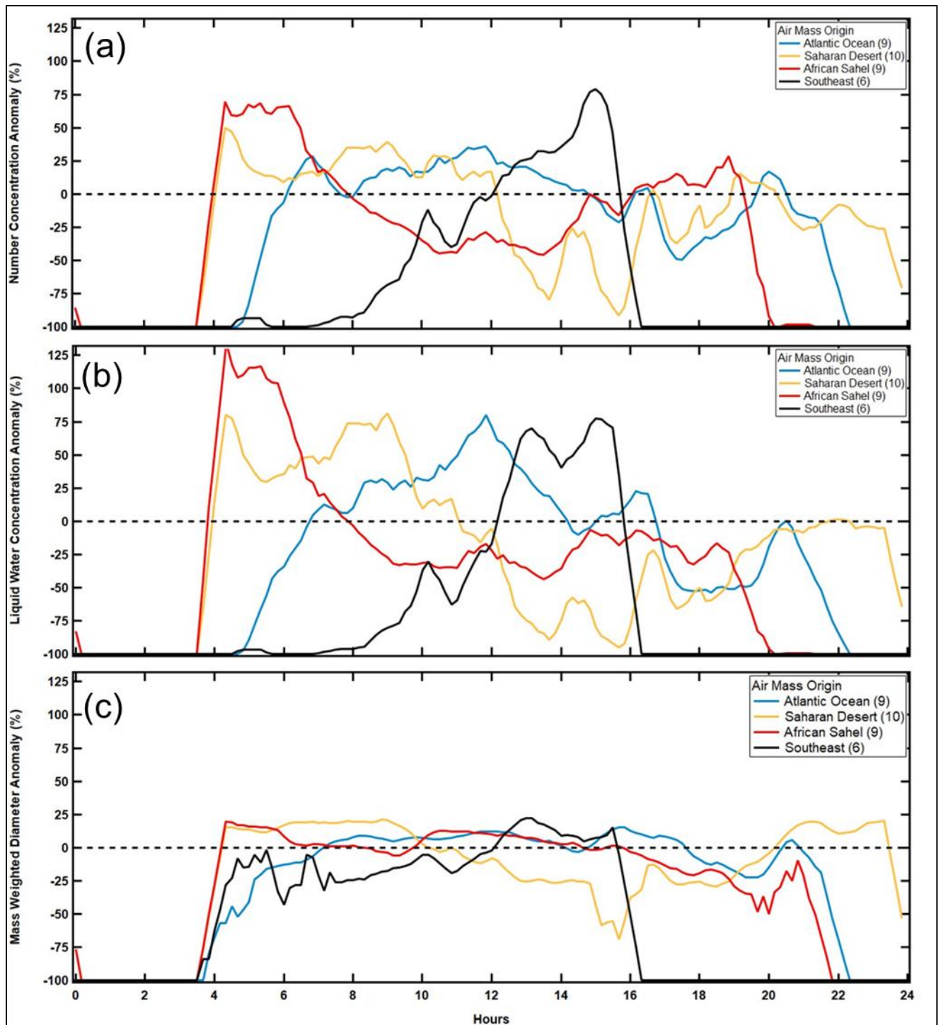
395 Figure 7. The deviations in a) number concentration, b) LWC and c) MVD from their average values over the time period of air mass intrusion are summarized in these figures for air mass types, in percent change.
