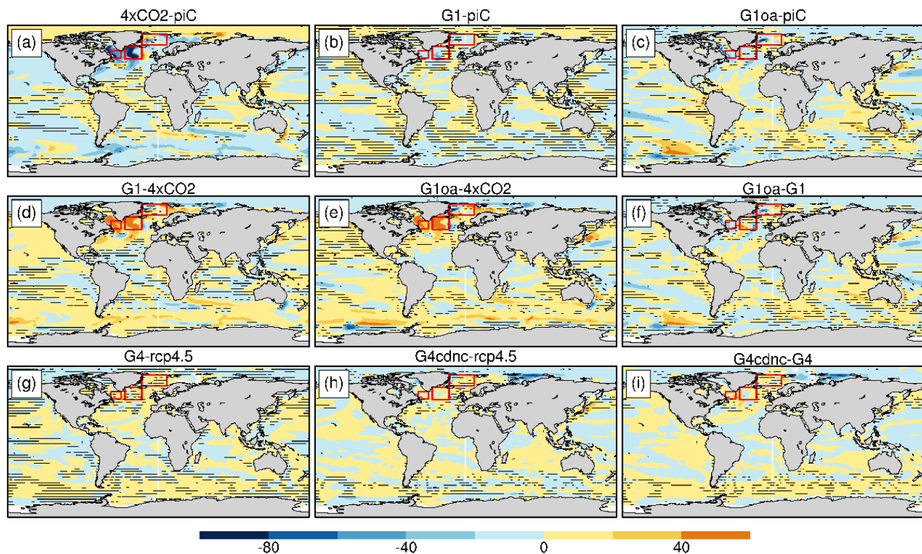
270 Figure 6: Upward heat flux change ( \text{W m}^{-2} ) in different scenarios(11-50yr). The red boxes mark the three deep convective regions in the northern North Atlantic (from left to right: Labrador, Irminger, and Norwegian seas, (often referred to as the Greenland-Iceland-Norwegian (GIN) Seas). Yellow to orange colors represent an increase in heat flux from the ocean to the atmosphere. Stippling indicates regions where differences are not significant at the 95% level according to the Wilcoxon signed-rank test.
